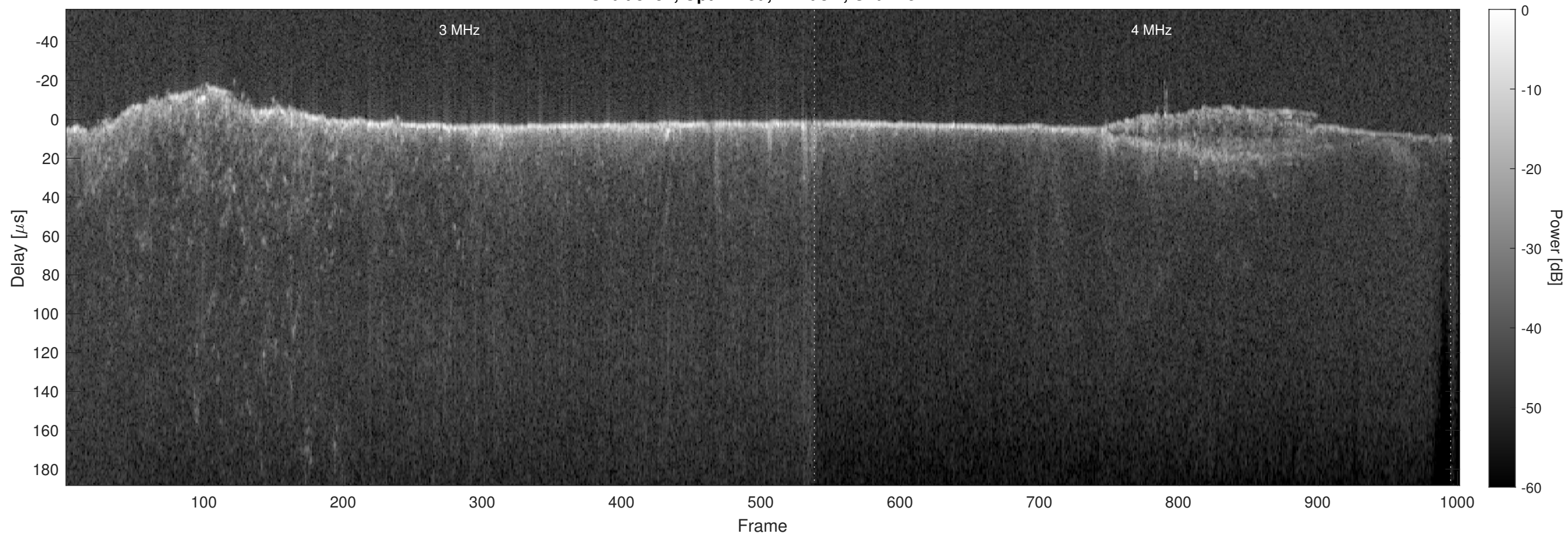
Orbit 5754, Optimized, Window, Channel 2
