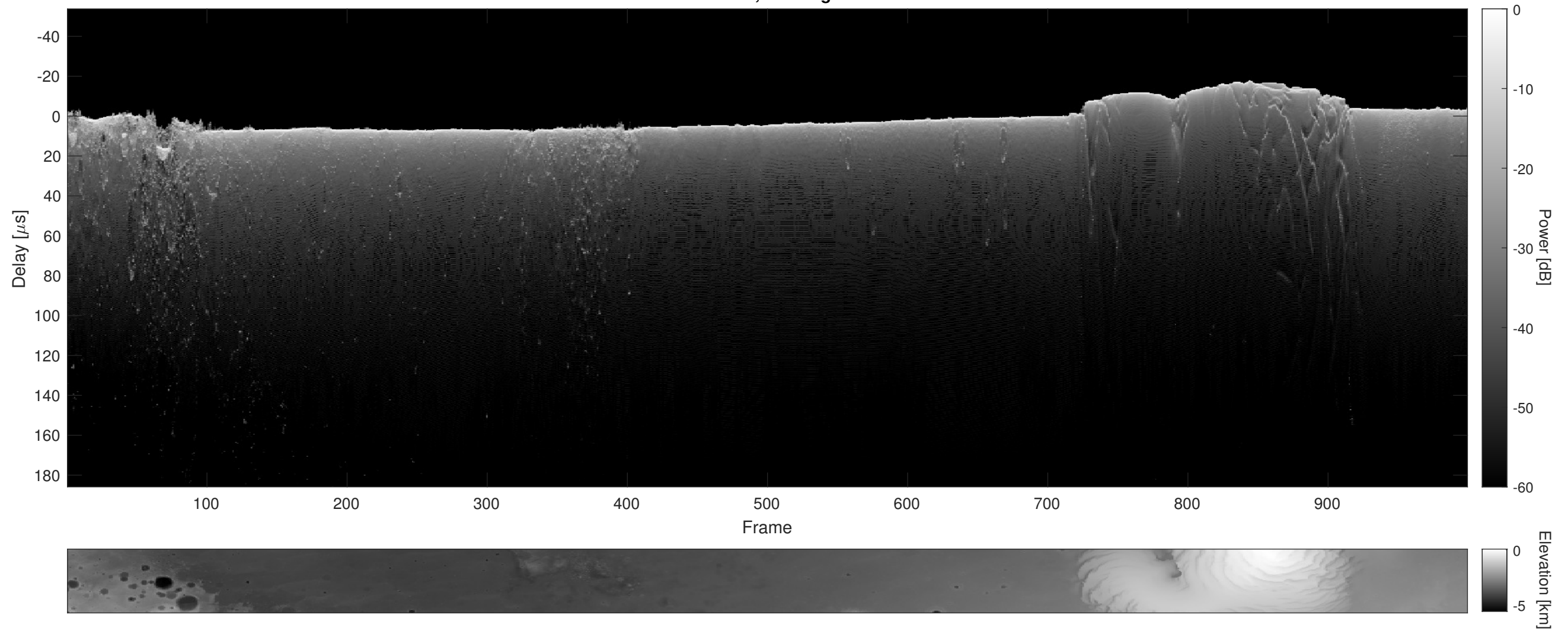
Orbit 5755, Cluttergram
