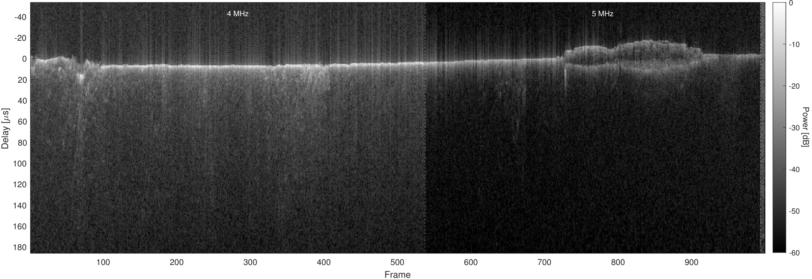
Orbit 5755, Optimized, No Window, Channel 2
