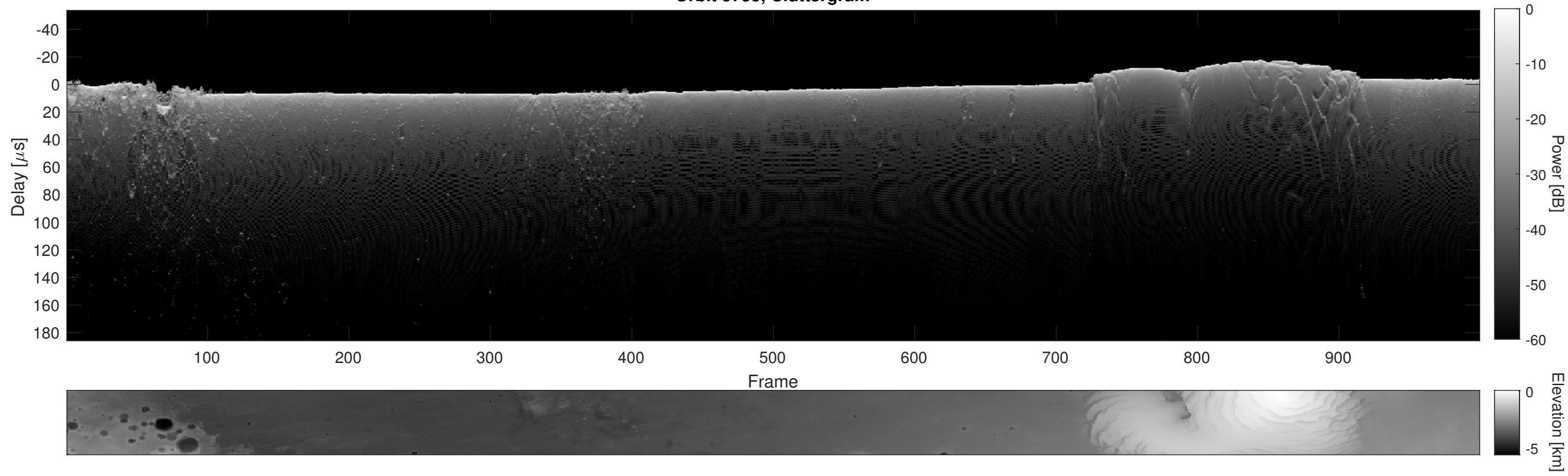
Orbit 5755, Cluttergram
