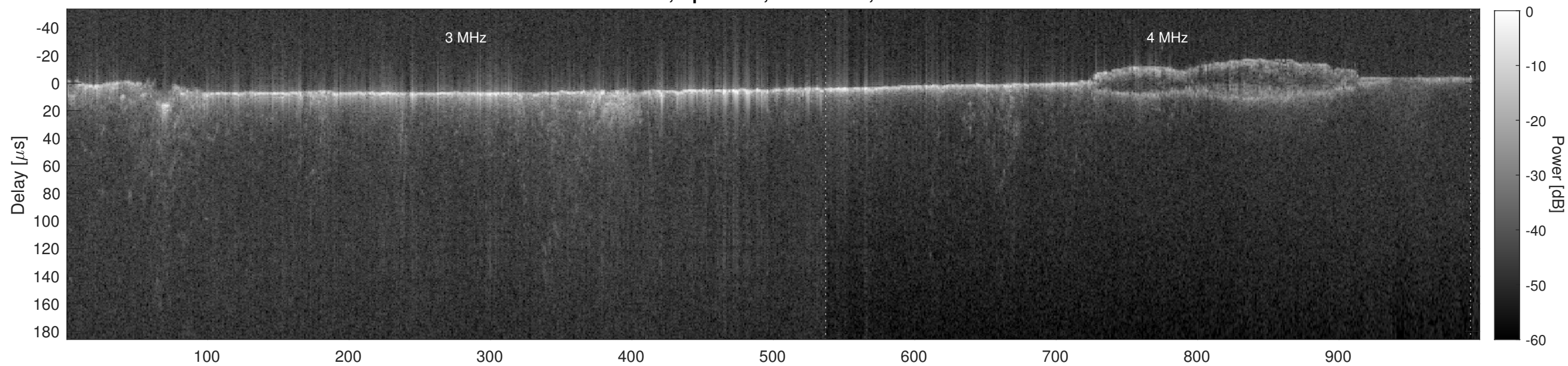
Orbit 5755, Cluttergram
