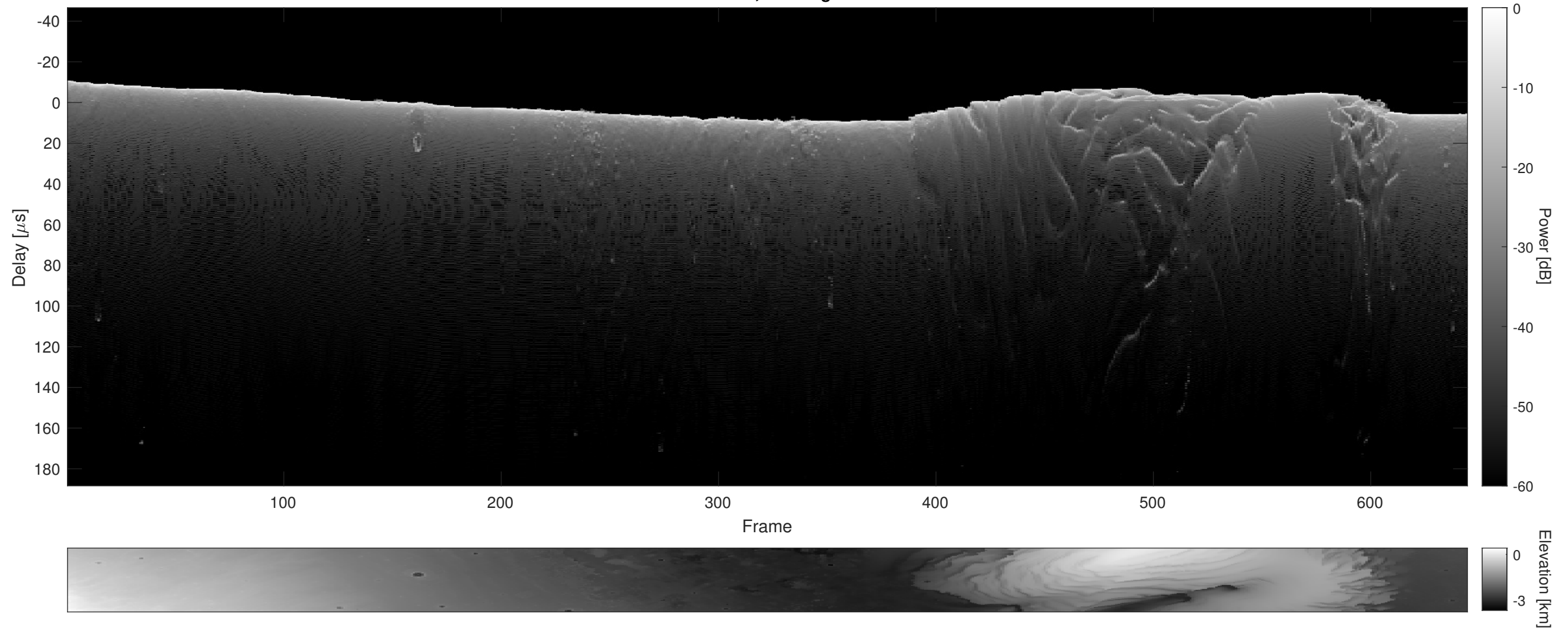
Orbit 5756, Cluttergram
