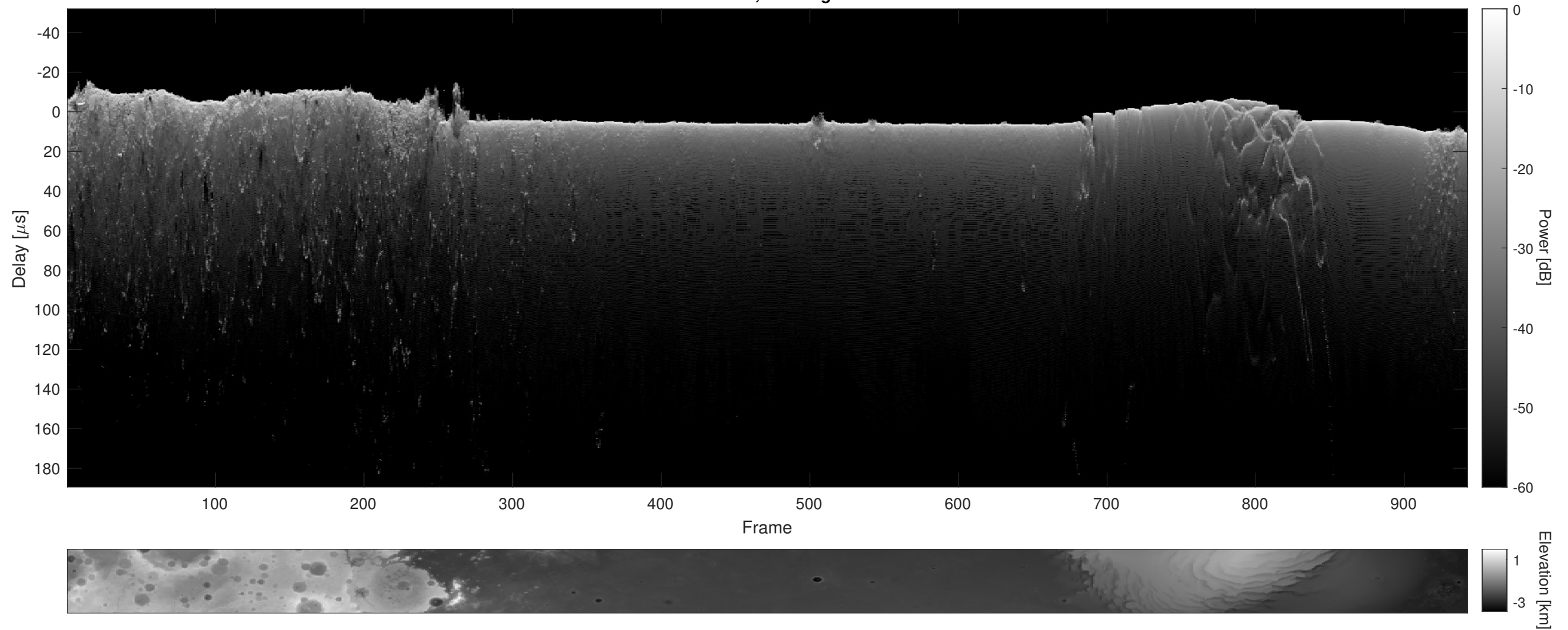
Orbit 5758, Cluttergram
