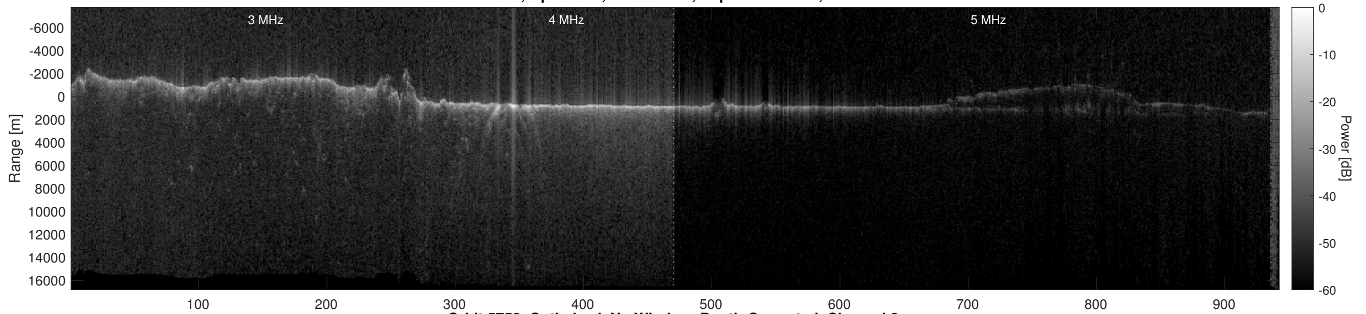
Orbit 5758, Optimized, No Window, Depth-Corrected, Channel 2
