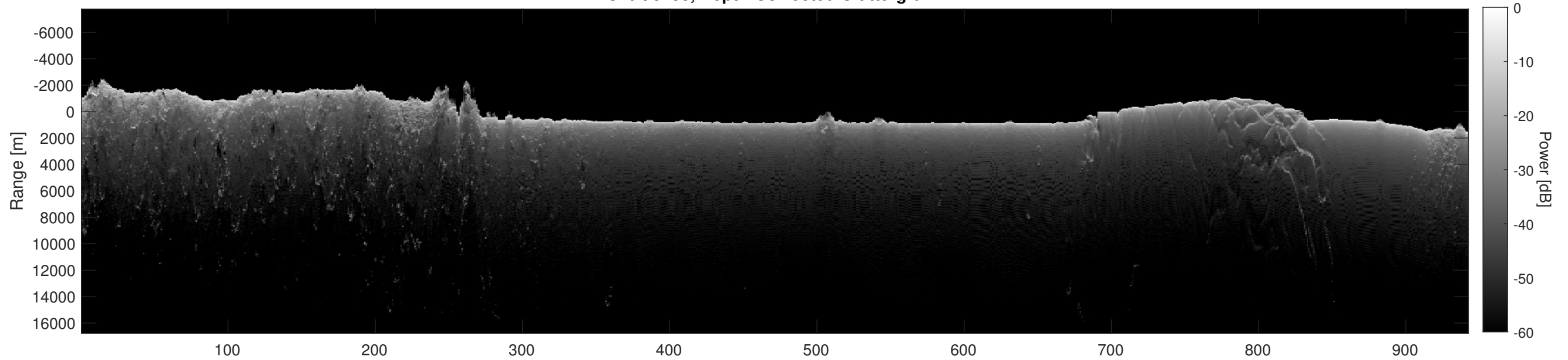
Orbit 5758, Depth-Corrected Cluttergram
