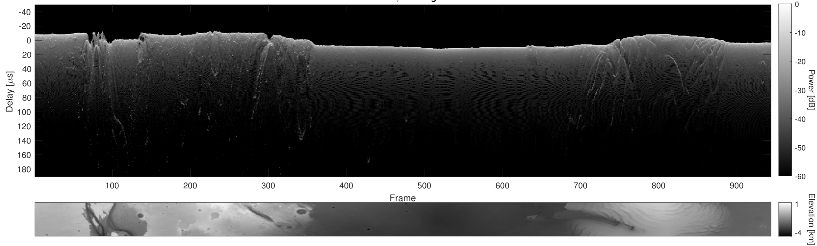
Orbit 5759, Cluttergram
