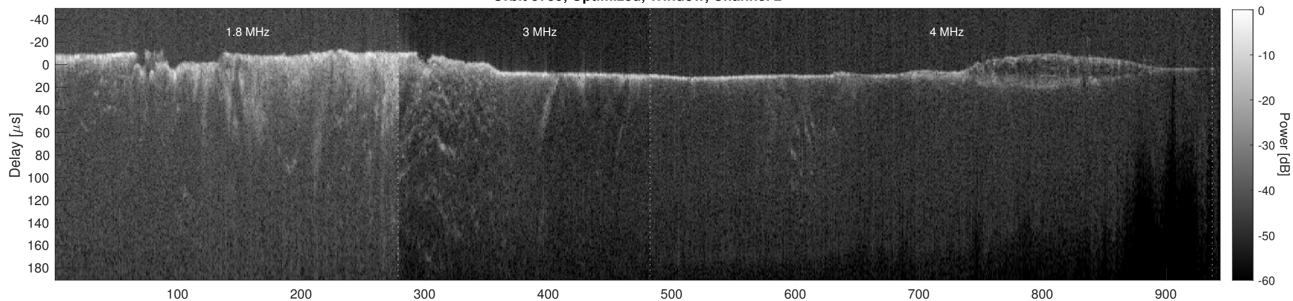
Orbit 5759, Cluttergram
