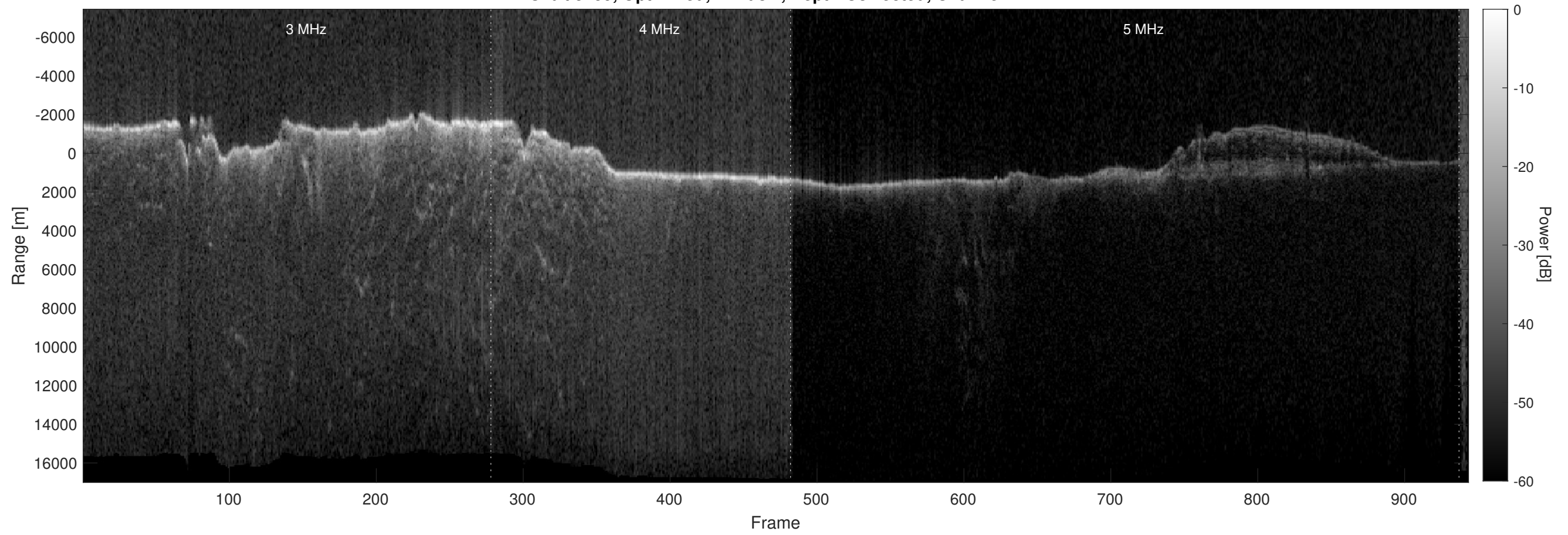
Orbit 5759, Optimized, Window, Depth-Corrected, Channel 2
