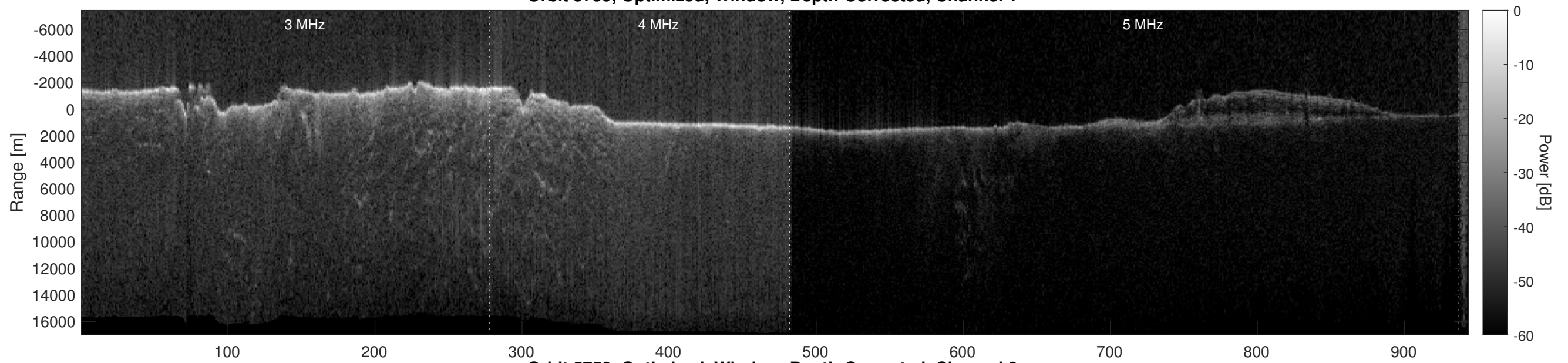
Orbit 5759, Optimized, Window, Depth-Corrected, Channel 2
