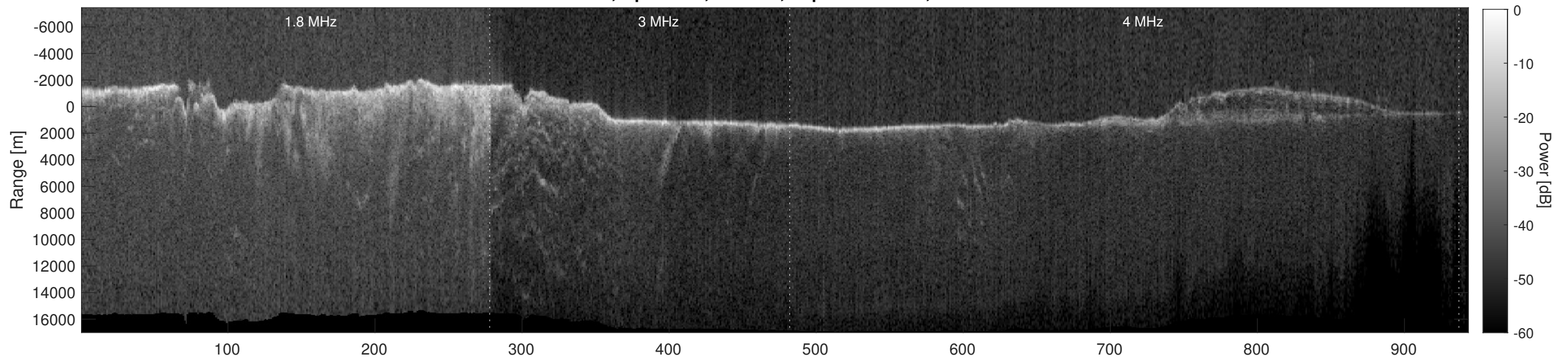
Orbit 5759, Depth-Corrected Cluttergram
