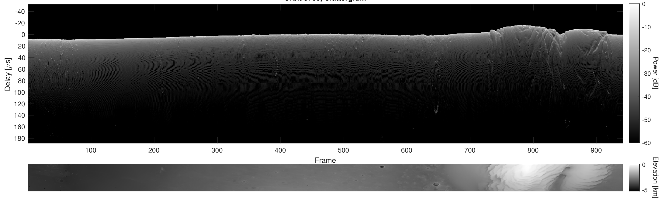
Orbit 5760, Cluttergram
