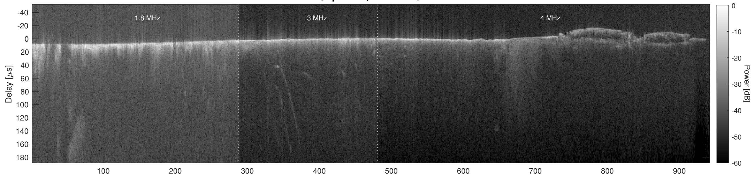
Orbit 5760, Cluttergram
