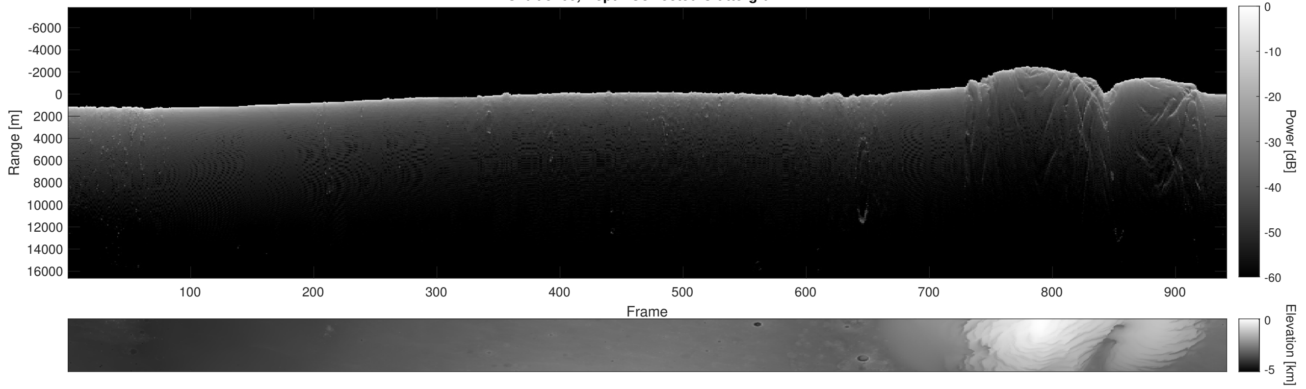
Orbit 5760, Depth-Corrected Cluttergram
