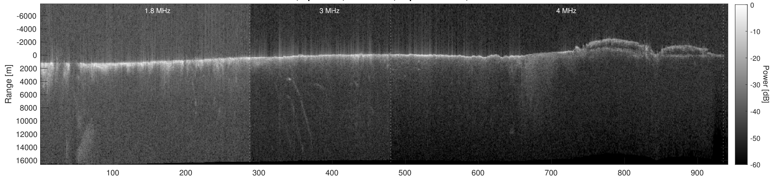
Orbit 5760, Depth-Corrected Cluttergram
