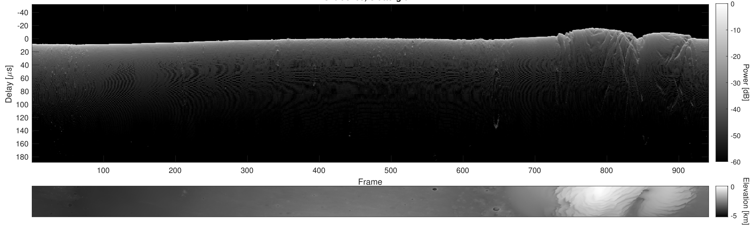
Orbit 5760, Cluttergram
