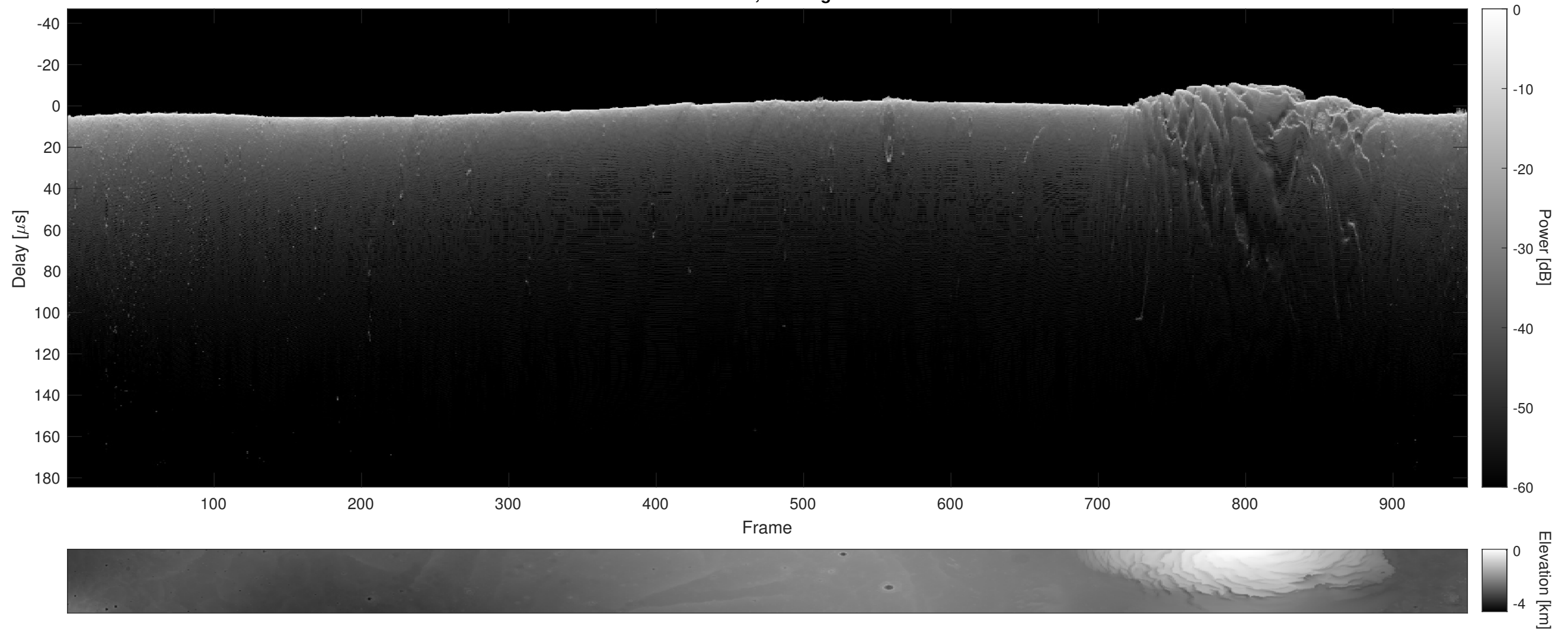
Orbit 5761, Cluttergram
