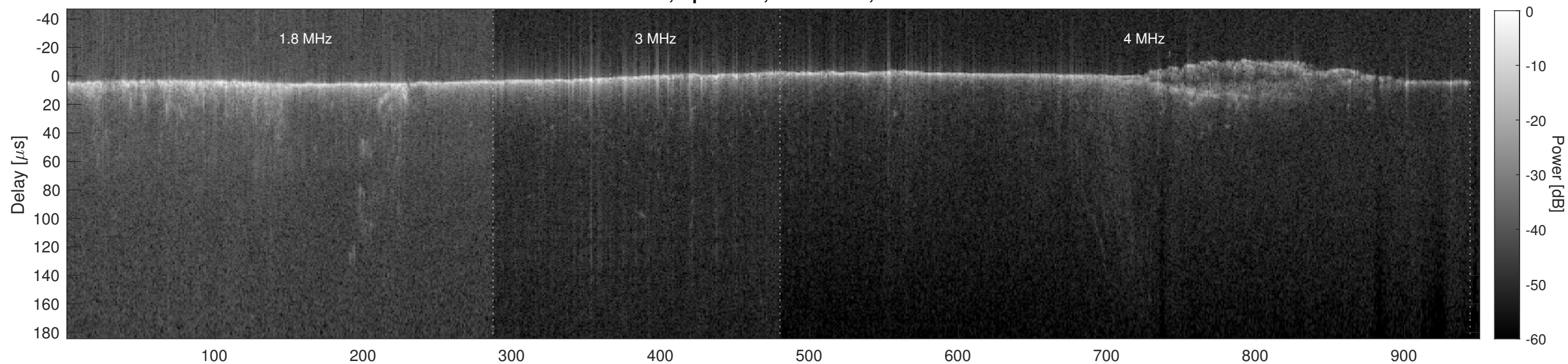
Orbit 5761, Cluttergram
