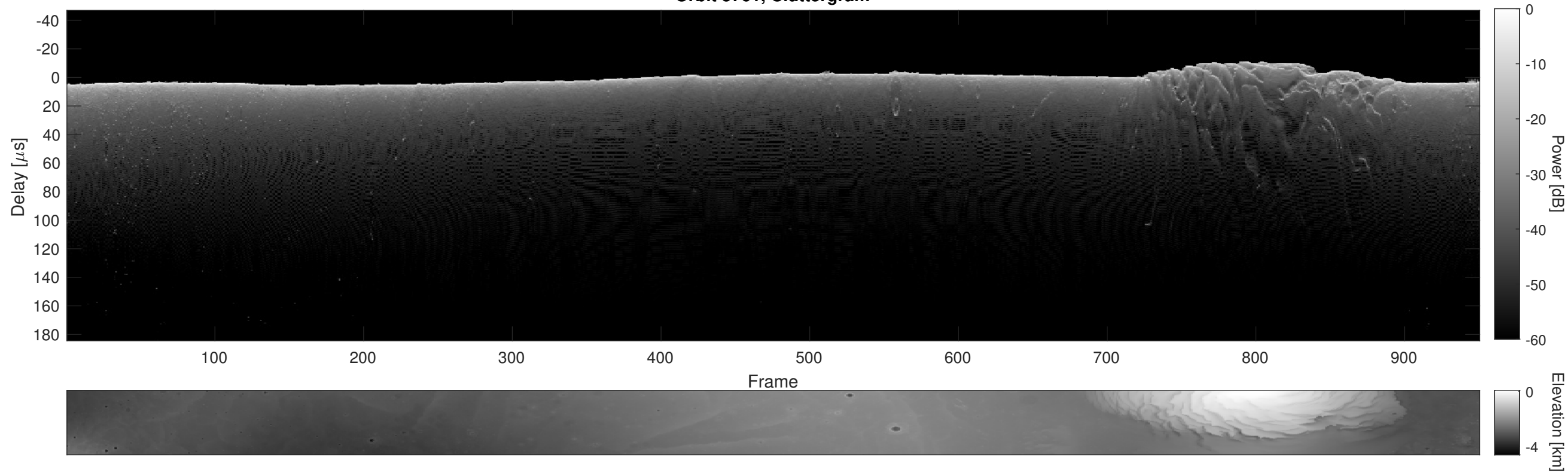
Orbit 5761, Cluttergram
