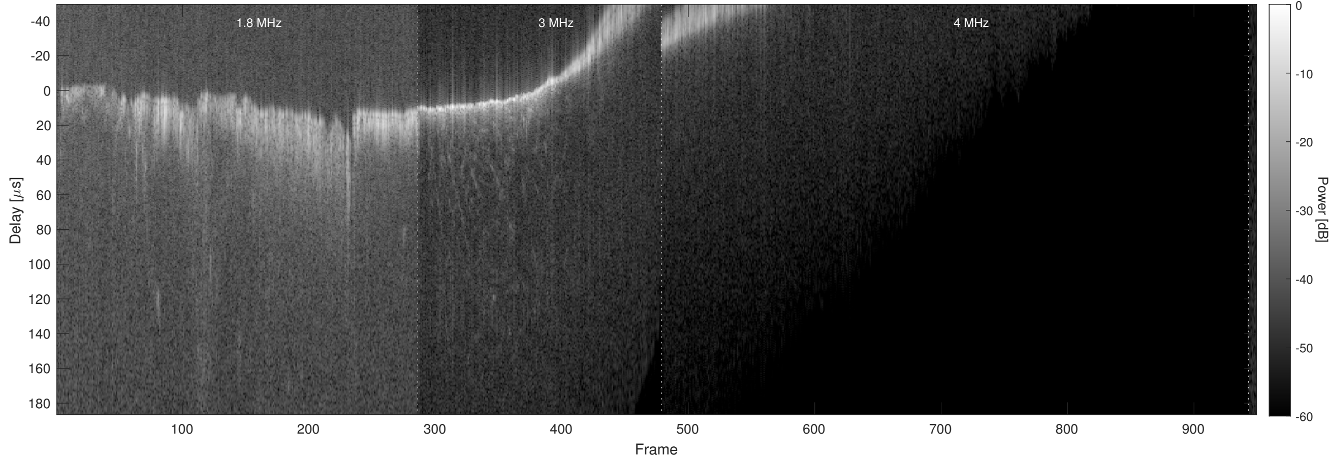
Orbit 5762, Chapman, No Window, Channel 2
