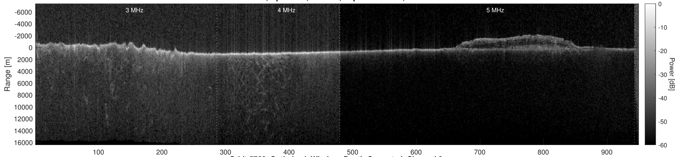
Orbit 5762, Optimized, Window, Depth-Corrected, Channel 2
