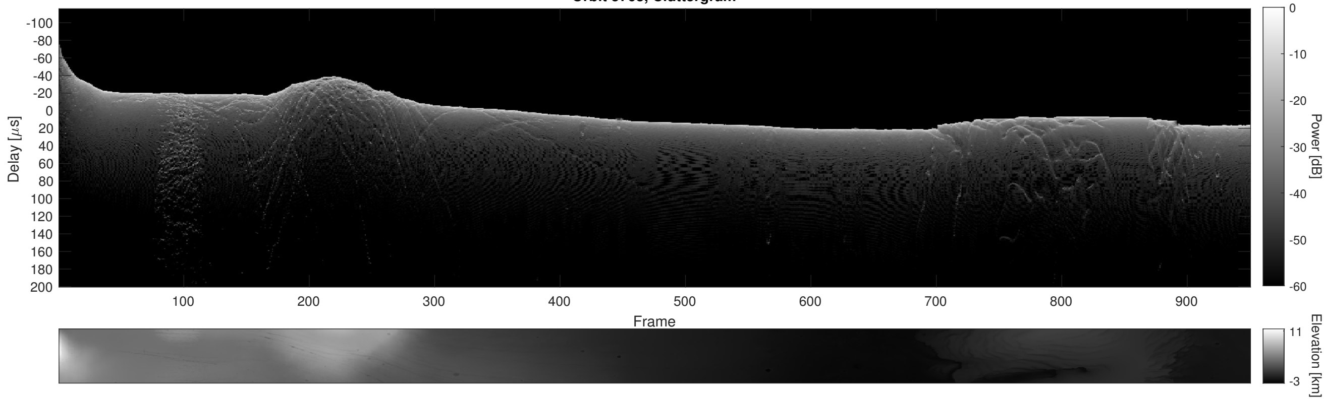
Orbit 5763, Cluttergram
