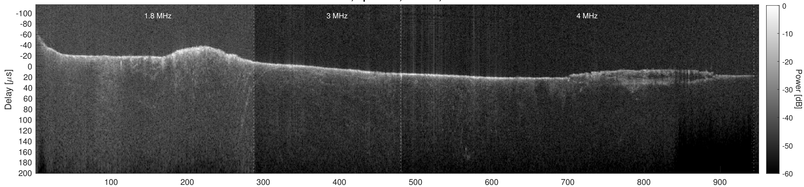
Orbit 5763, Cluttergram
