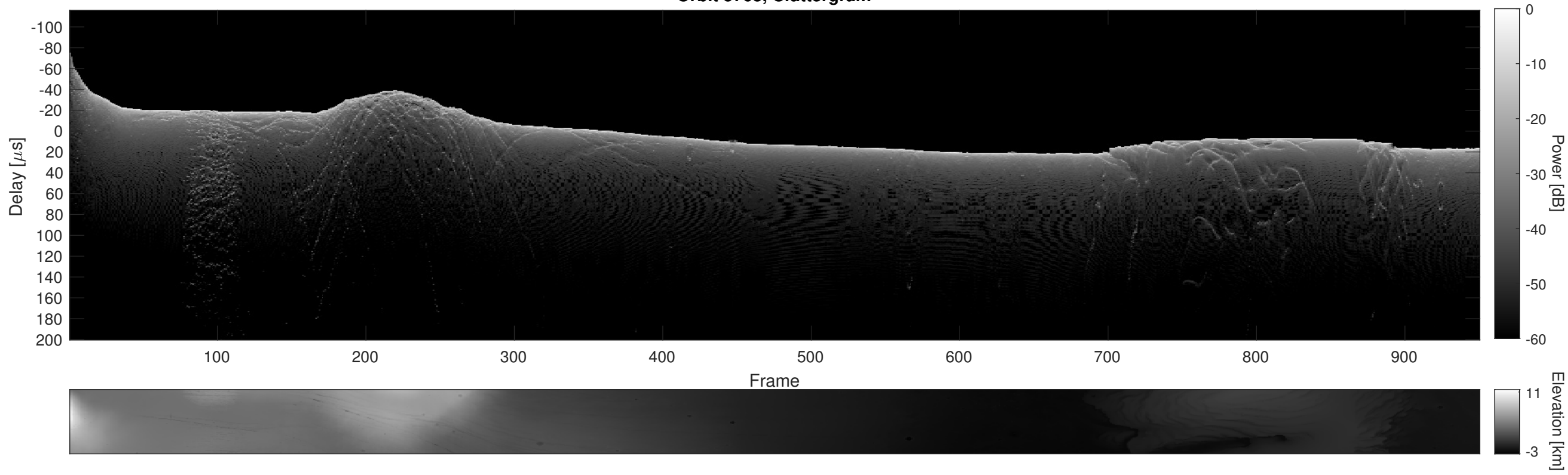
Orbit 5763, Cluttergram
