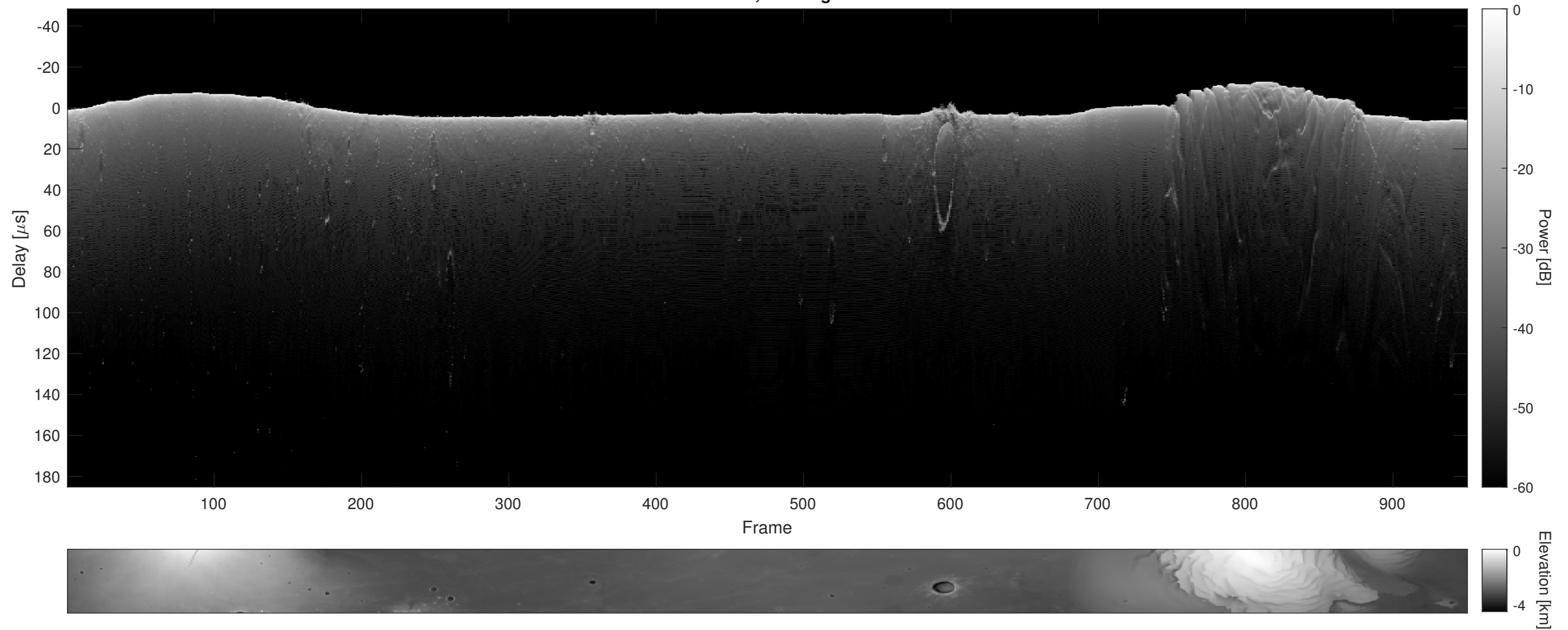
Orbit 5764, Cluttergram
