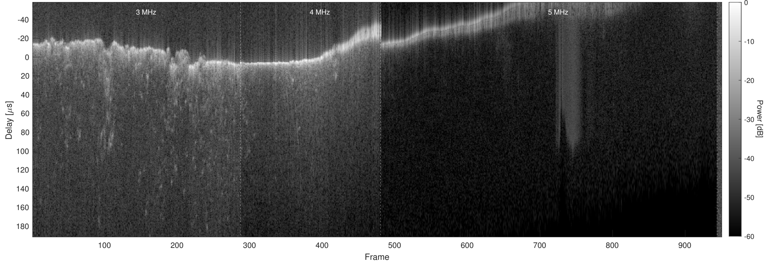
Orbit 5765, Chapman, No Window, Channel 2
