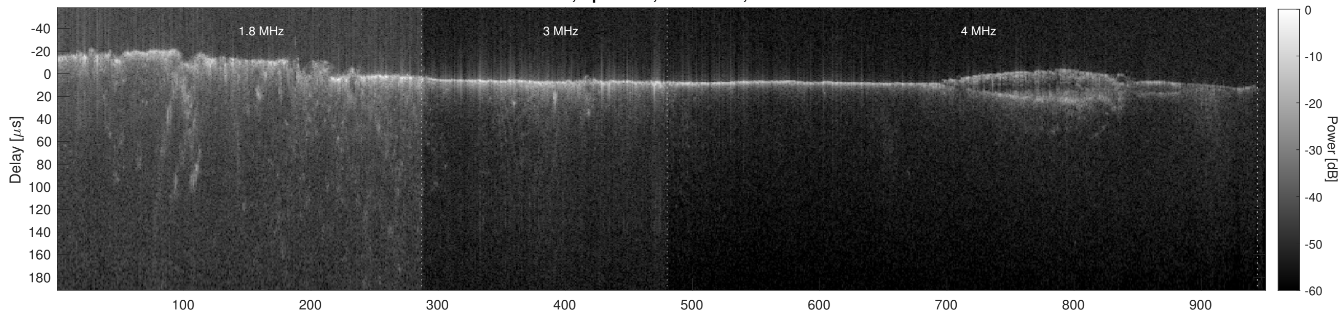
Orbit 5765, Cluttergram
