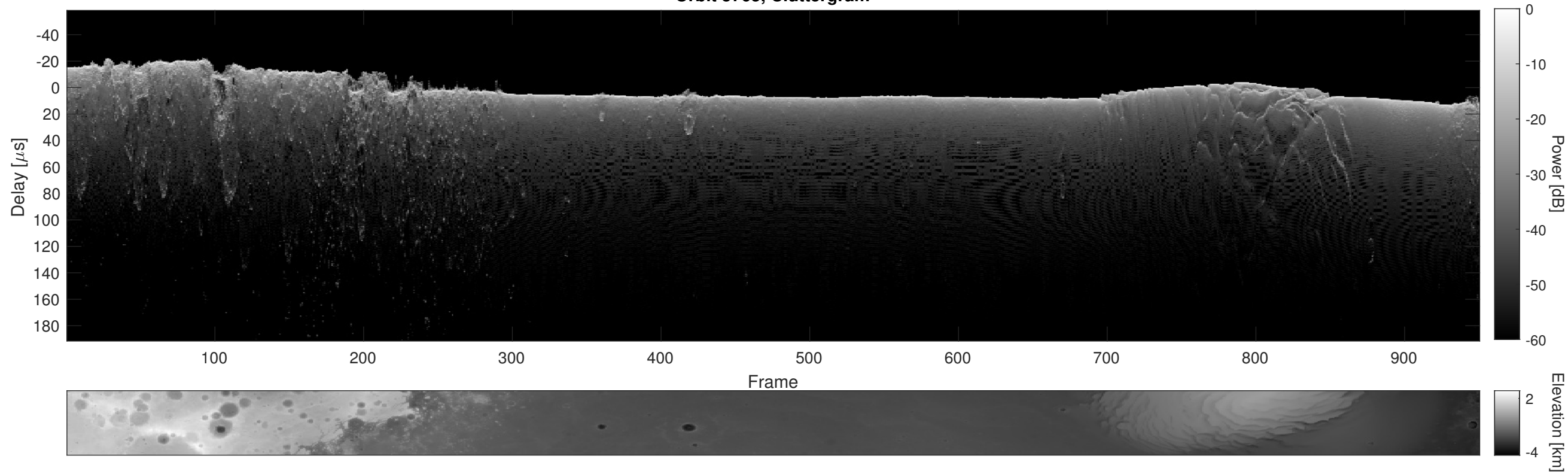
Orbit 5765, Cluttergram
