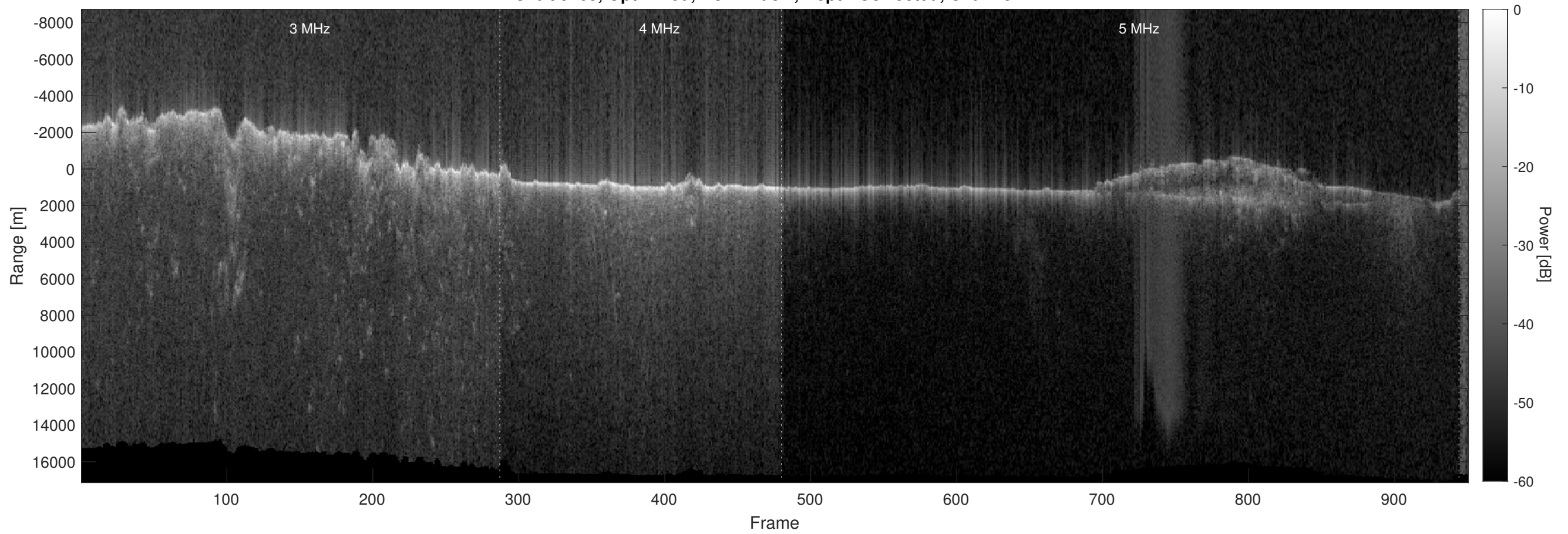
Orbit 5765, Optimized, No Window, Depth-Corrected, Channel 2
