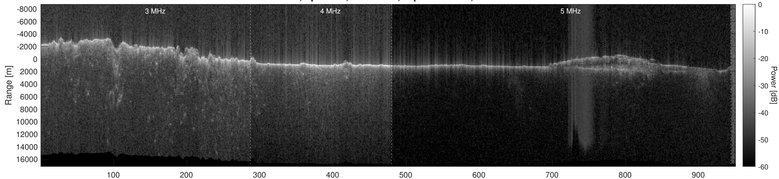
Orbit 5765, Optimized, No Window, Depth-Corrected, Channel 2
