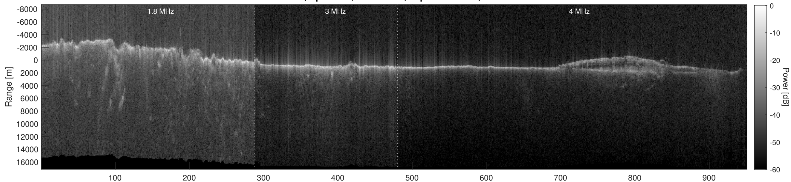
Orbit 5765, Depth-Corrected Cluttergram
