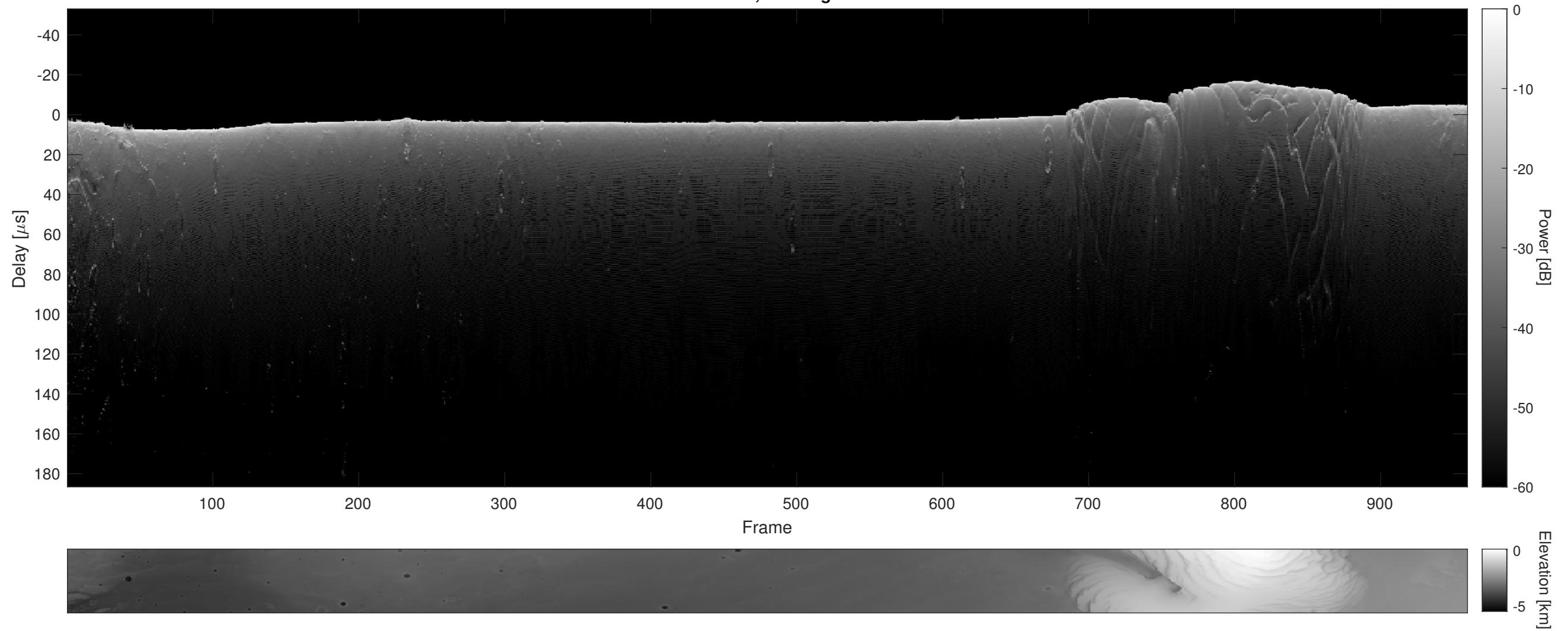
Orbit 5766, Cluttergram
