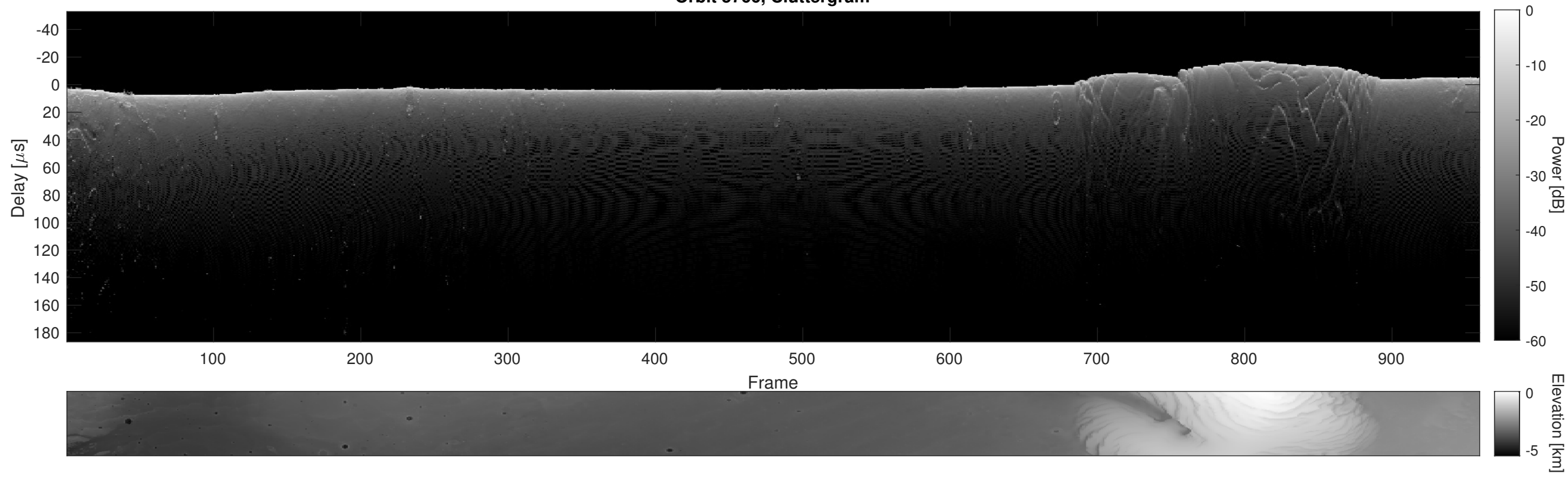
Orbit 5766, Cluttergram
