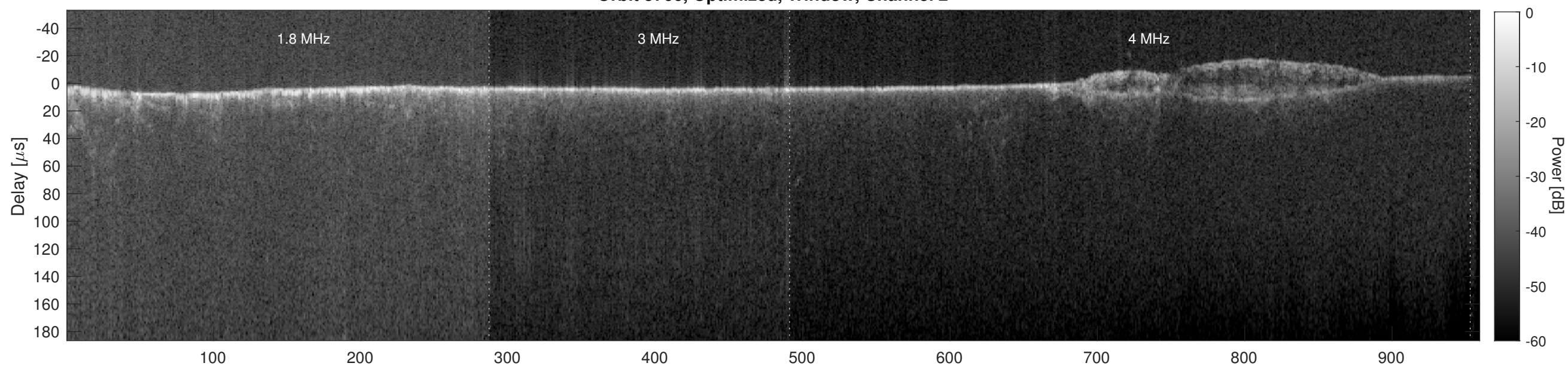
Orbit 5766, Cluttergram
