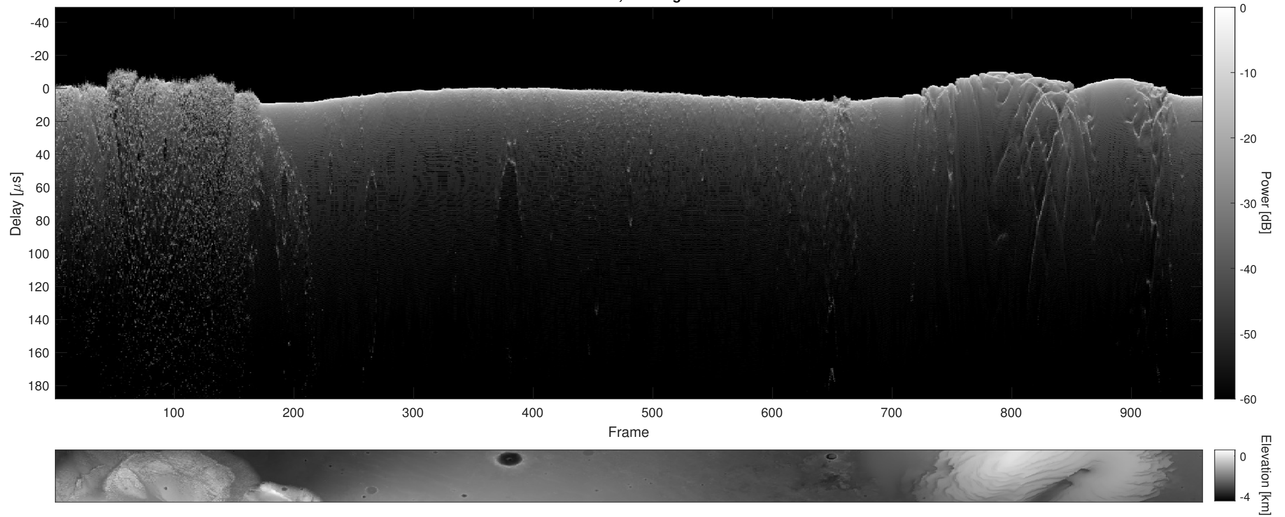
Orbit 5767, Cluttergram
