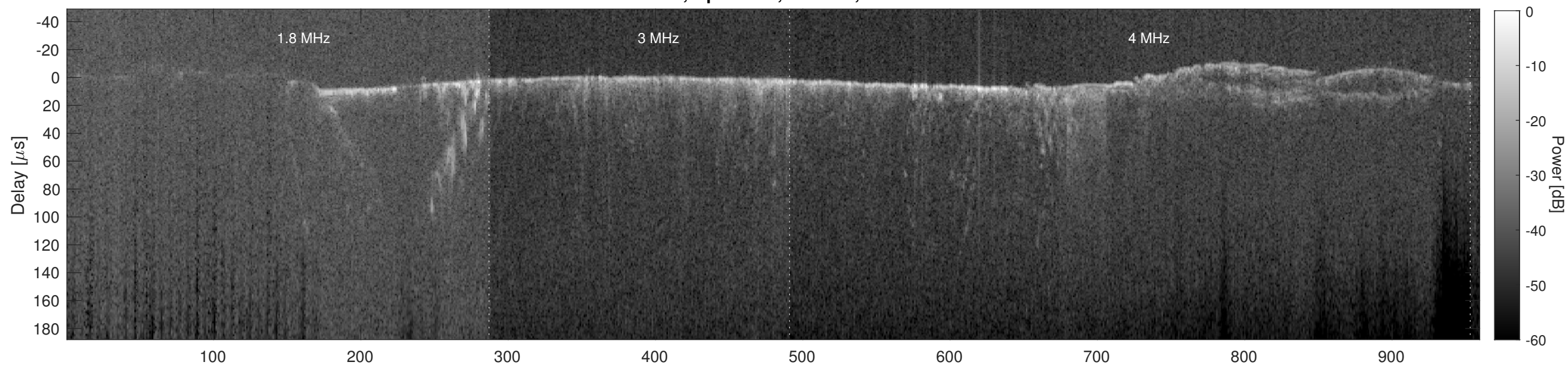
Orbit 5767, Cluttergram
