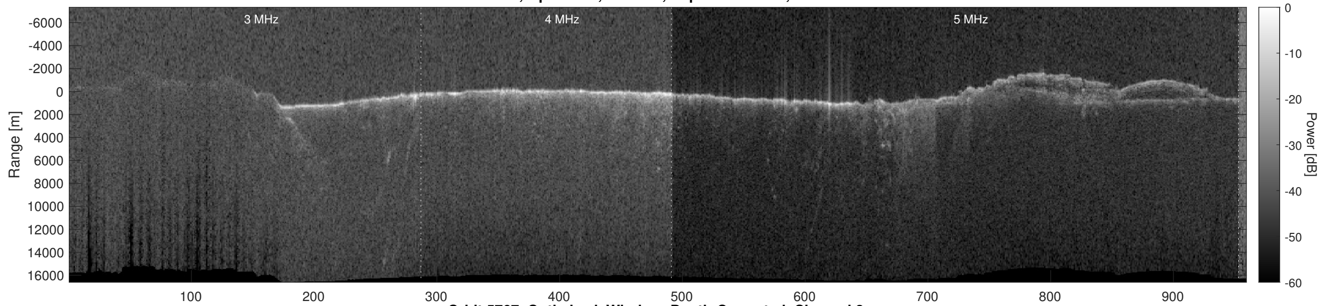
Orbit 5767, Optimized, Window, Depth-Corrected, Channel 2
