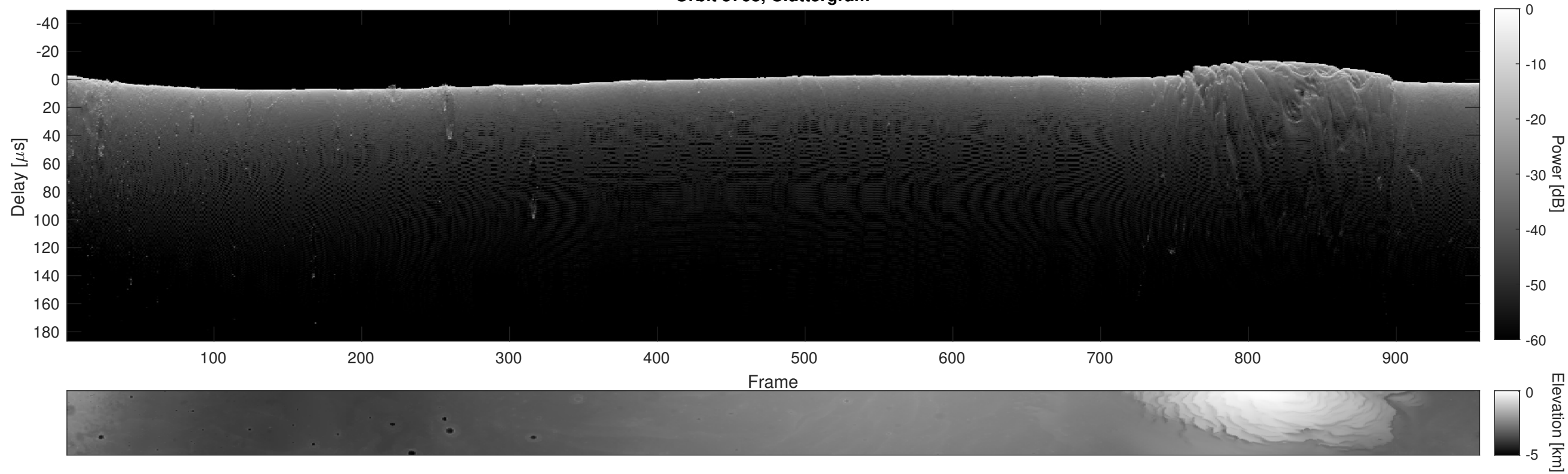
Orbit 5768, Cluttergram
