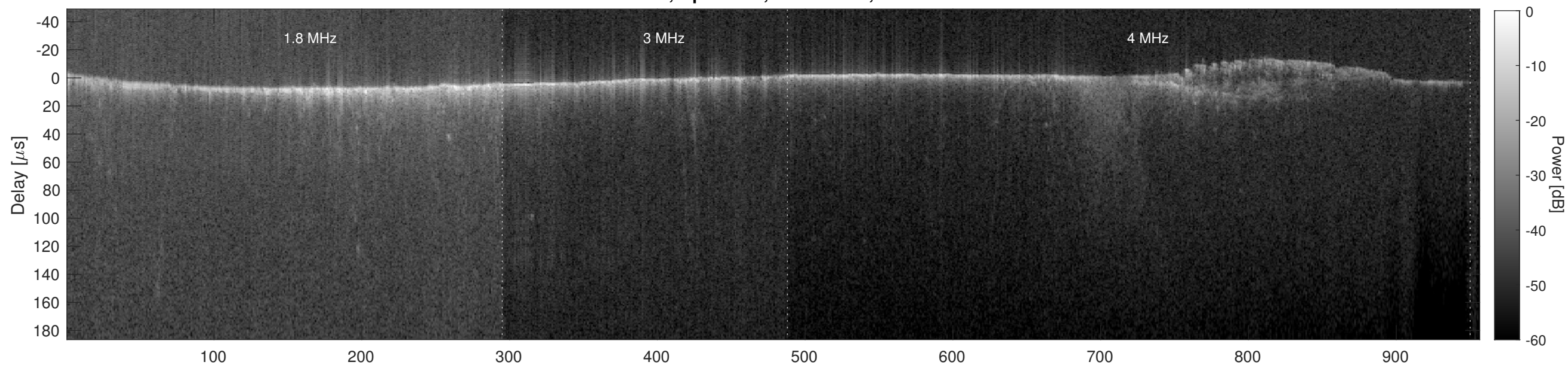
Orbit 5768, Cluttergram
