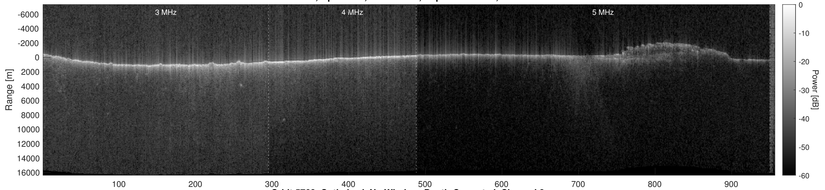
Orbit 5768, Optimized, No Window, Depth-Corrected, Channel 2
