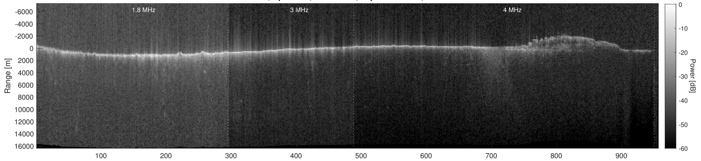
Orbit 5768, Depth-Corrected Cluttergram
