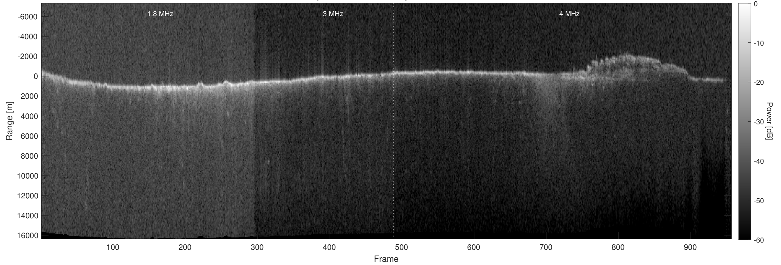
Orbit 5768, Optimized, Window, Depth-Corrected, Channel 2
