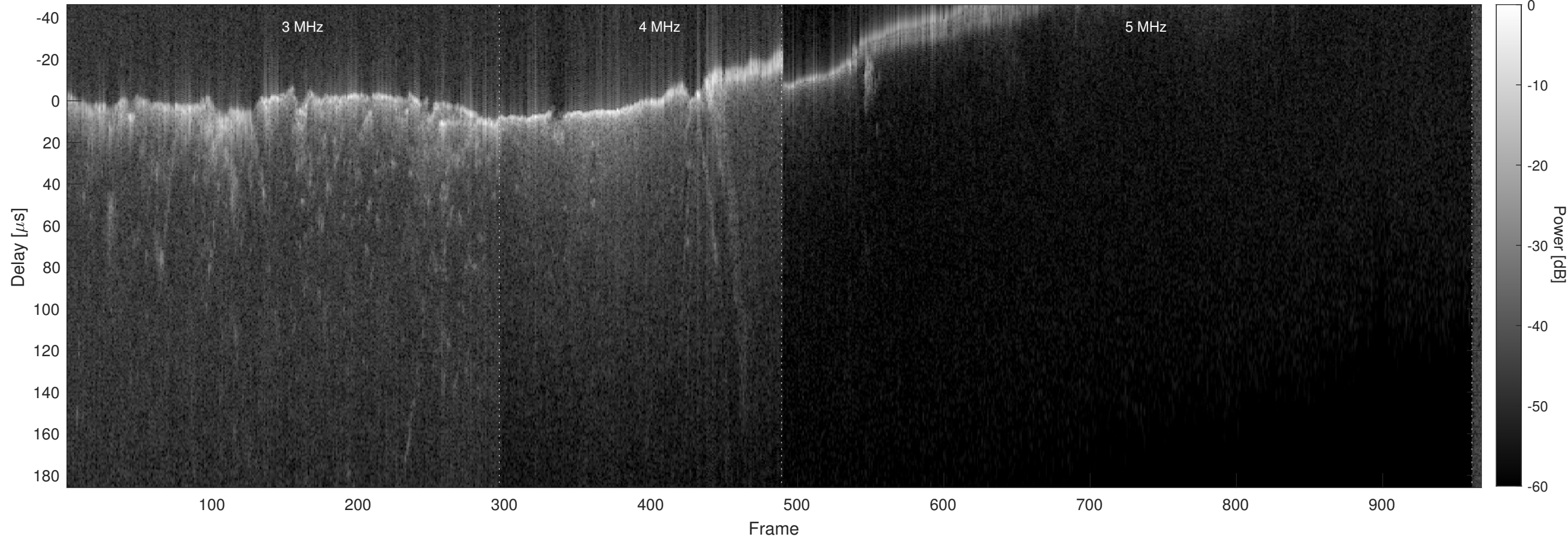
Orbit 5769, Chapman, No Window, Channel 2
