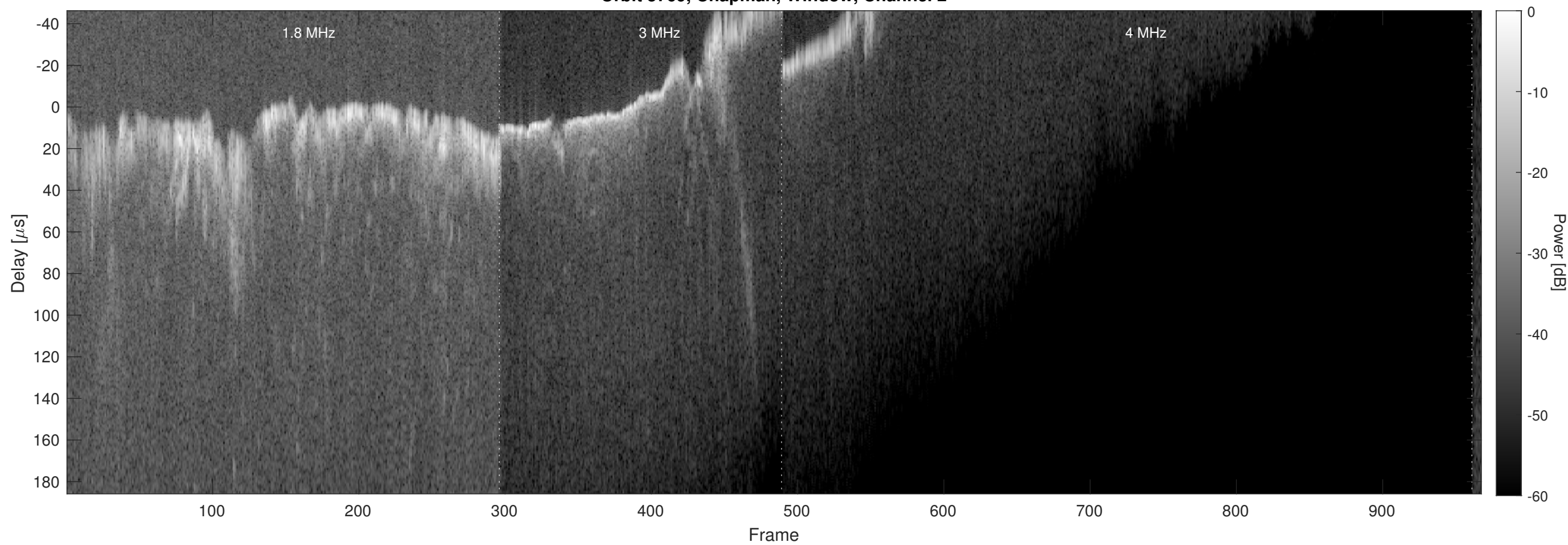
Orbit 5769, Chapman, Window, Channel 2
