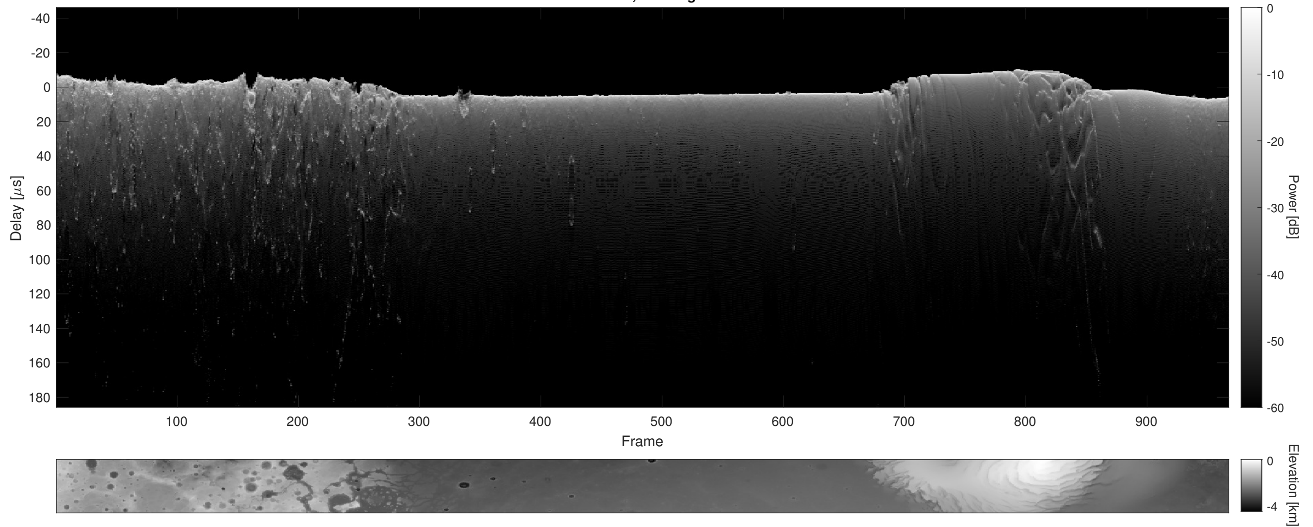
Orbit 5769, Cluttergram
