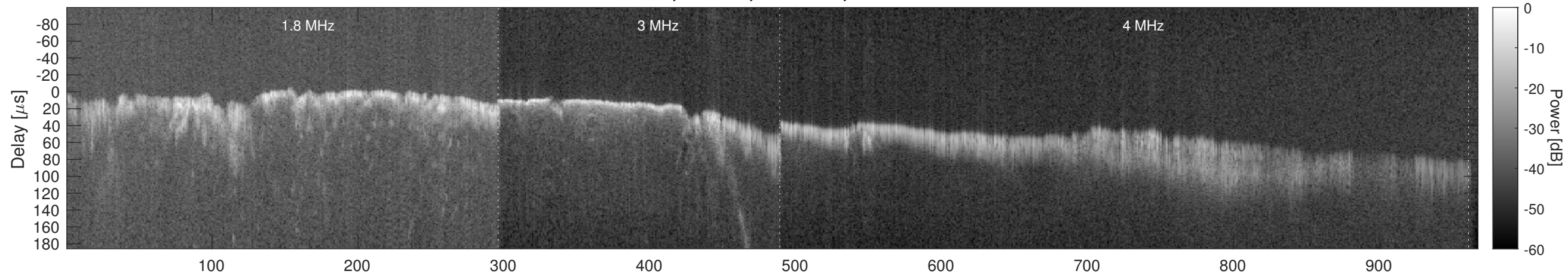
Orbit 5769, Window, Channel 2, Chapman
