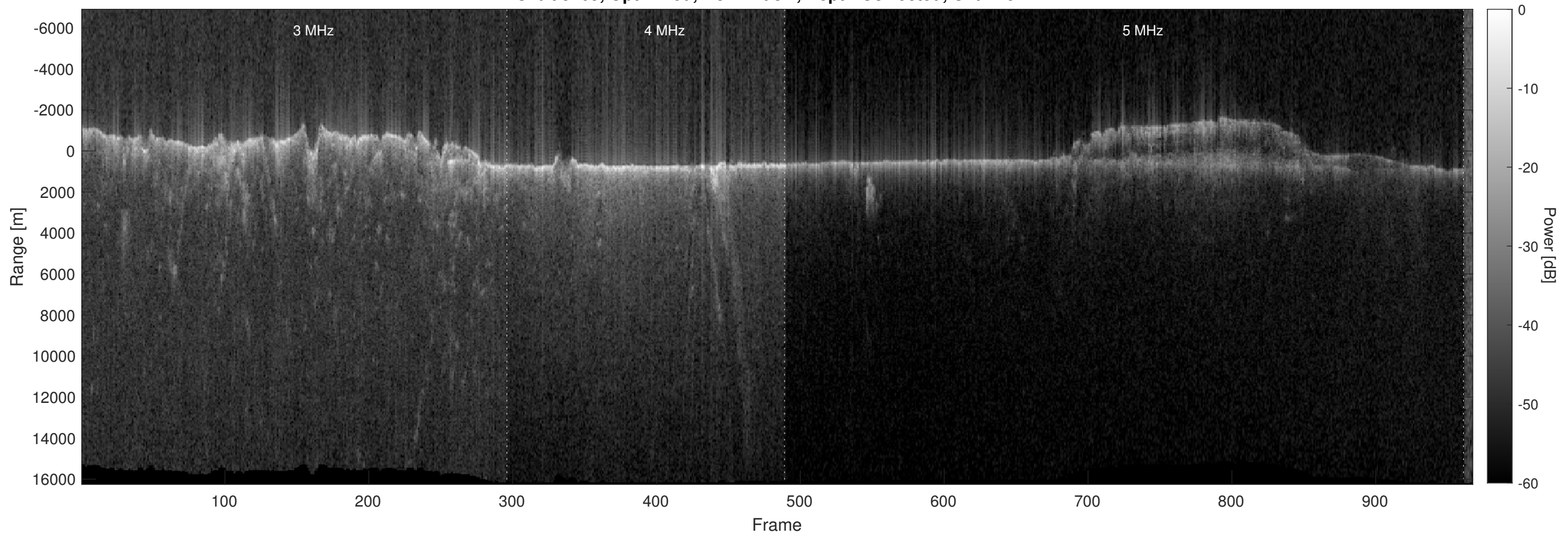
Orbit 5769, Optimized, No Window, Depth-Corrected, Channel 2
