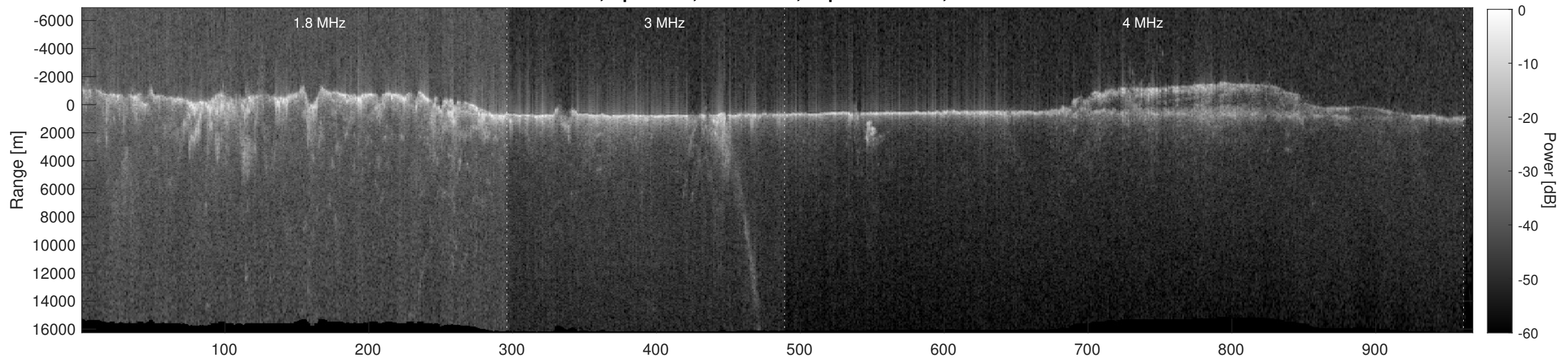
Orbit 5769, Depth-Corrected Cluttergram
