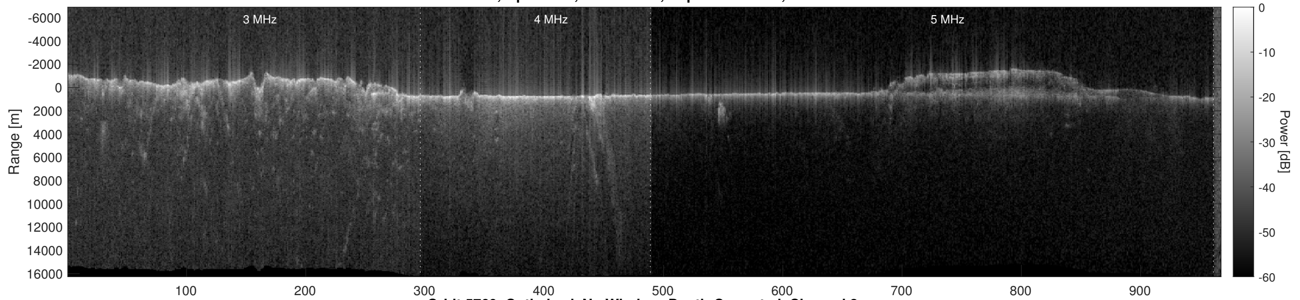
Orbit 5769, Optimized, No Window, Depth-Corrected, Channel 2
