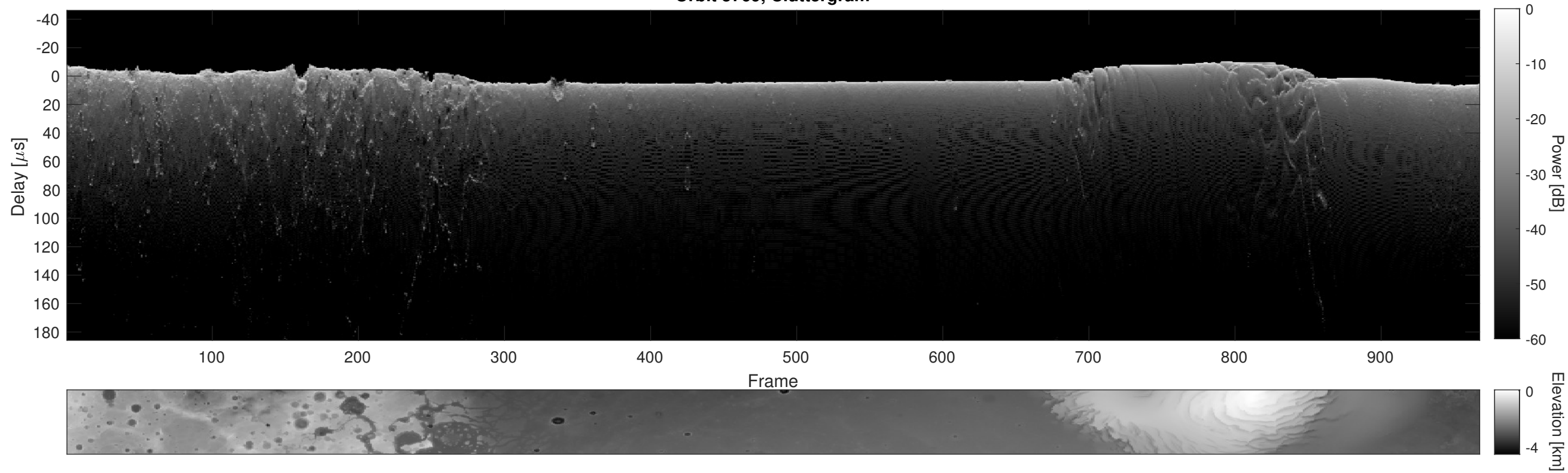
Orbit 5769, Cluttergram
