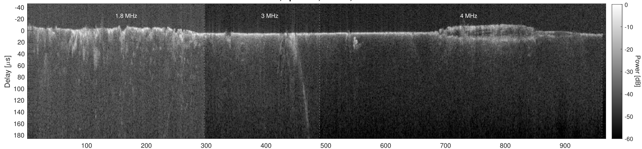
Orbit 5769, Cluttergram
