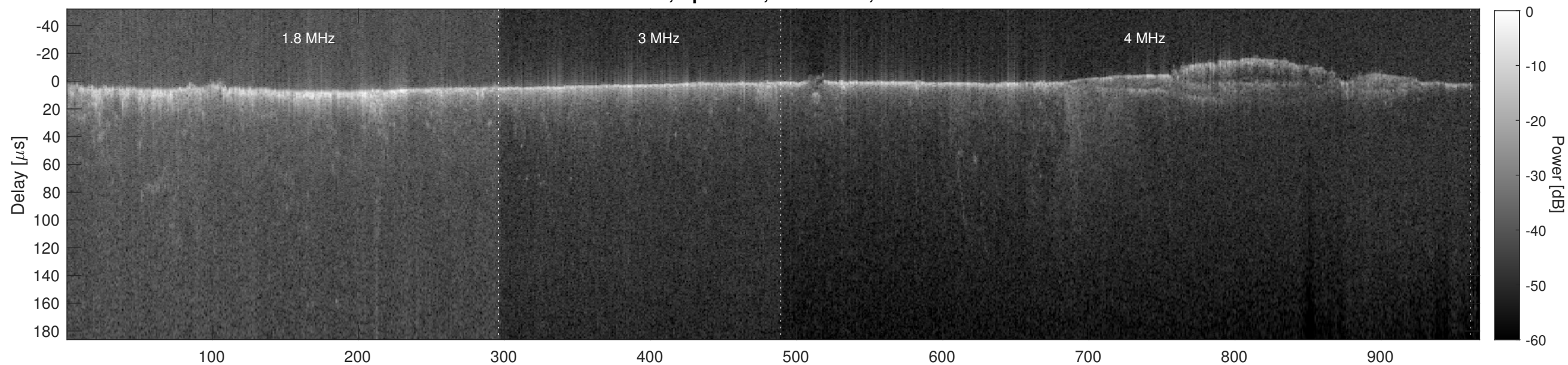
Orbit 5771, Cluttergram
