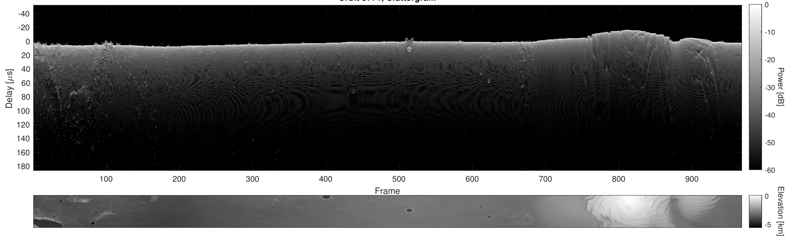
Orbit 5771, Cluttergram
