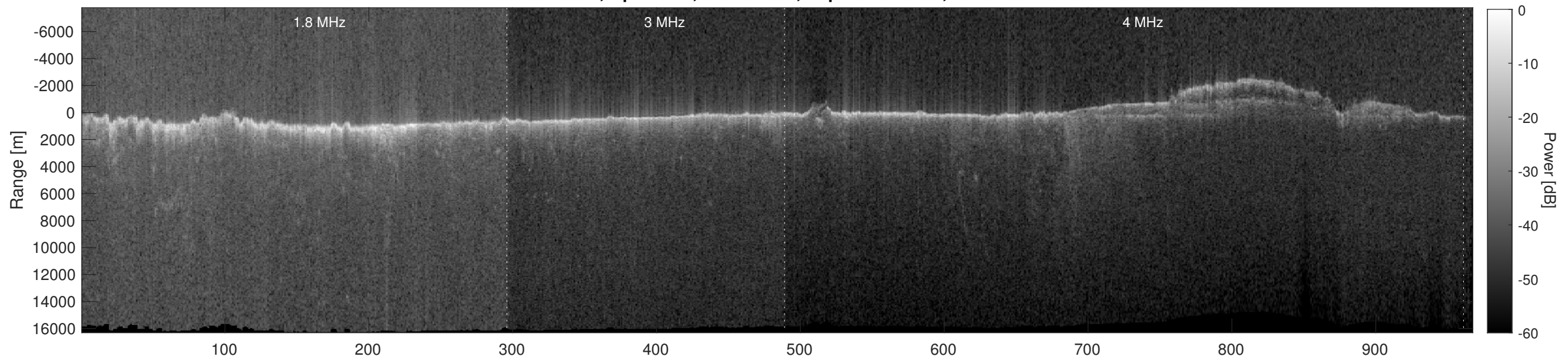
Orbit 5771, Depth-Corrected Cluttergram
