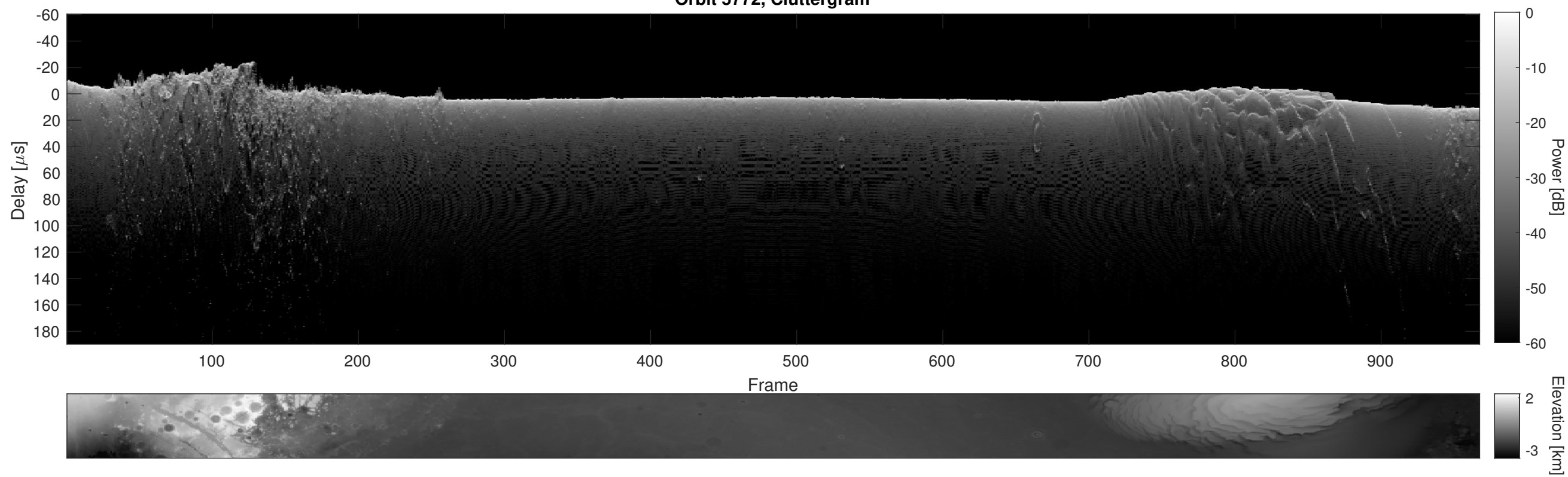
Orbit 5772, Cluttergram
