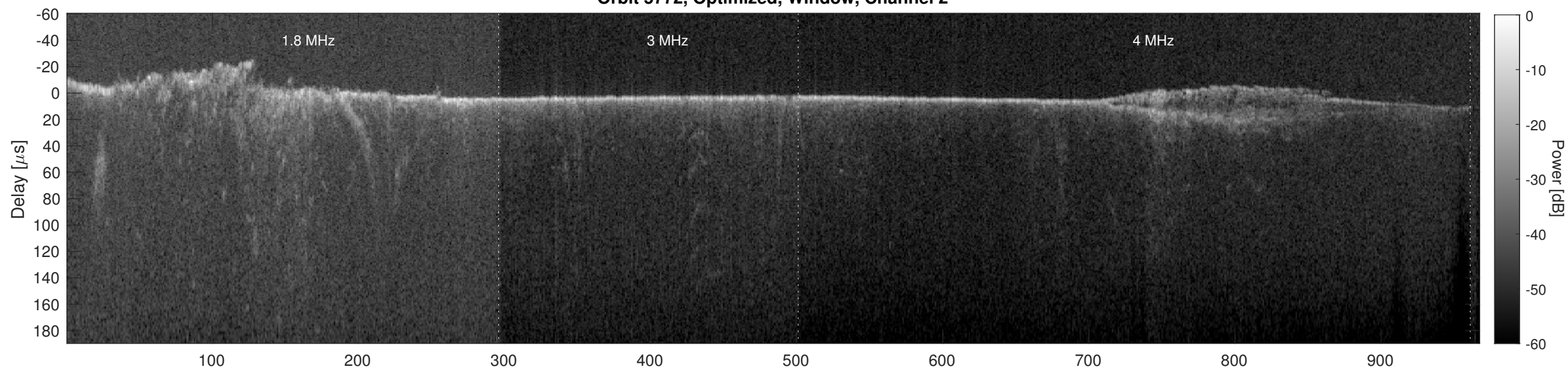
Orbit 5772, Cluttergram
