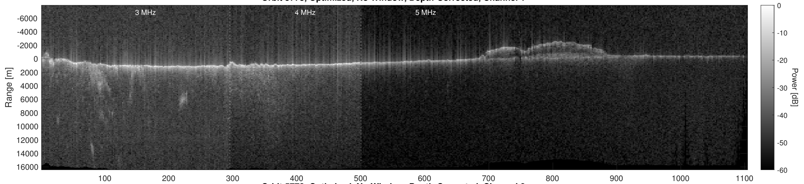
Orbit 5773, Optimized, No Window, Depth-Corrected, Channel 2
