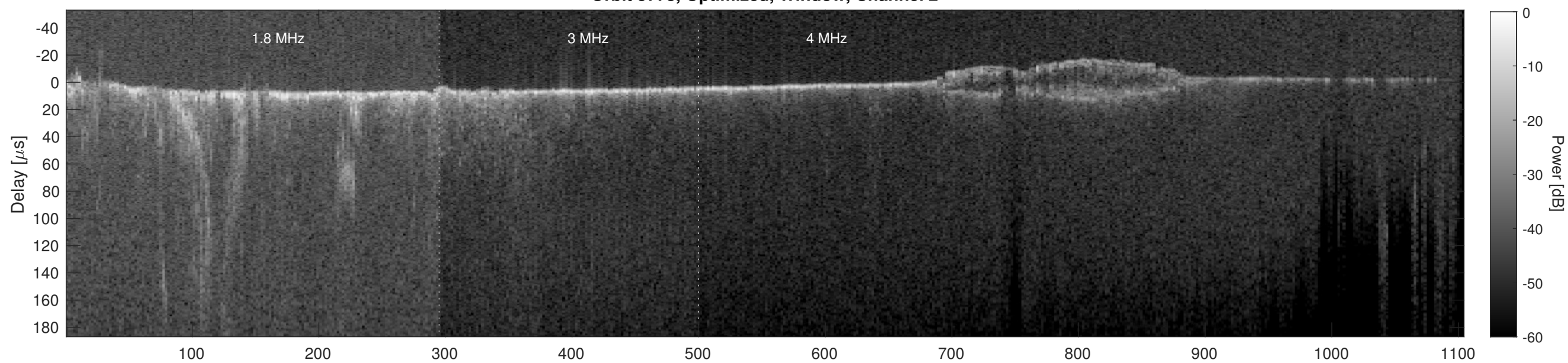
Orbit 5773, Cluttergram
