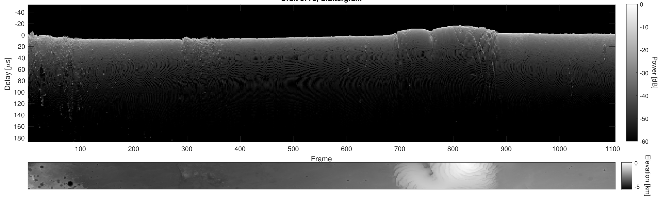
Orbit 5773, Cluttergram
