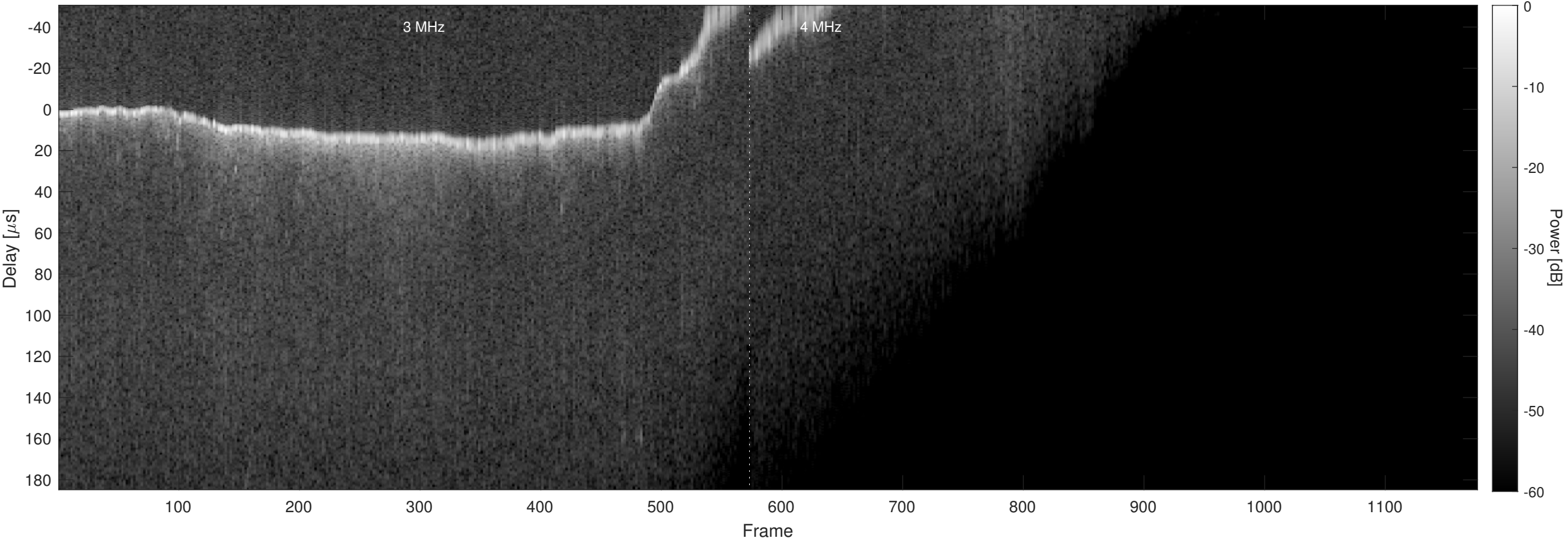
Orbit 5775, Chapman, Window, Channel 2
