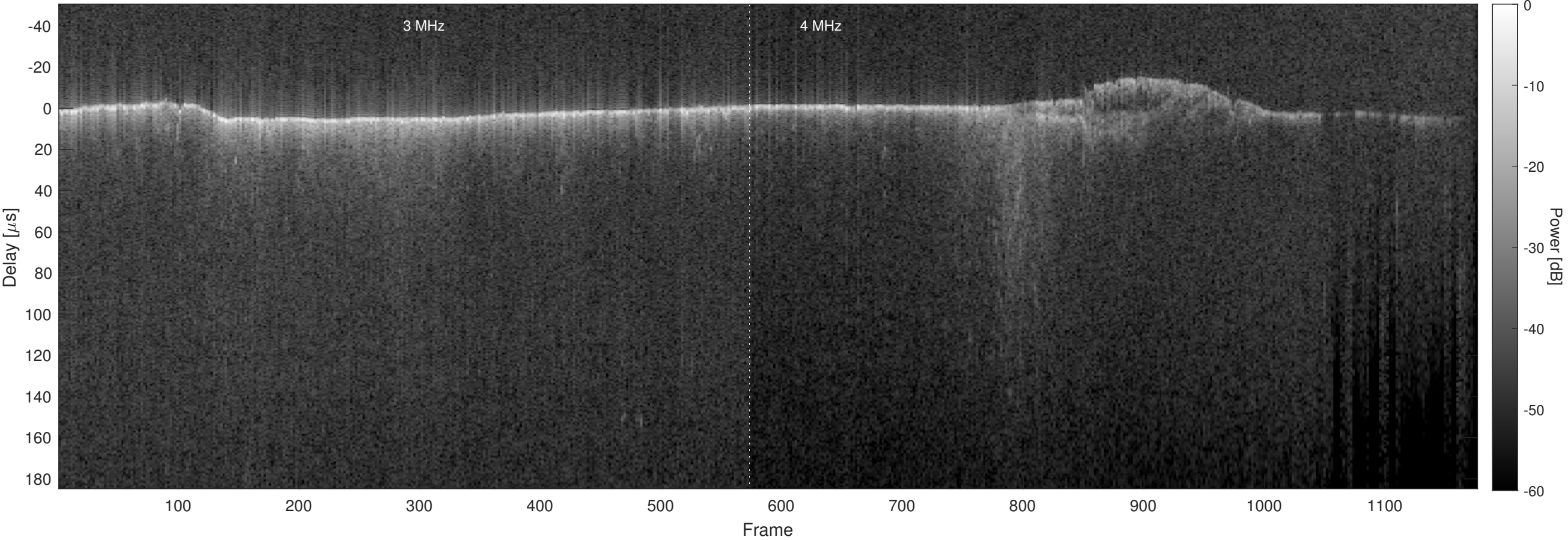
Orbit 5775, Optimized, No Window, Channel 2
