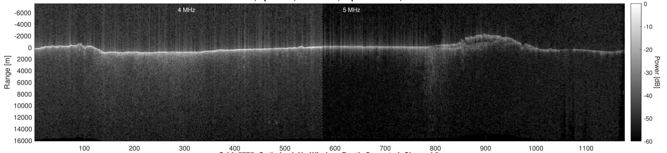
Orbit 5775, Optimized, No Window, Depth-Corrected, Channel 2
