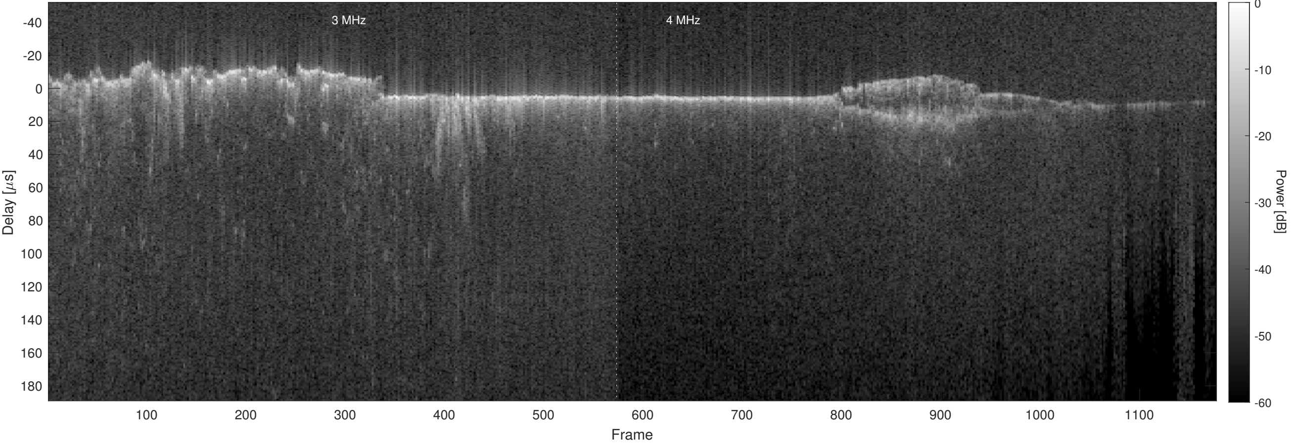
Orbit 5776, Optimized, No Window, Channel 2
