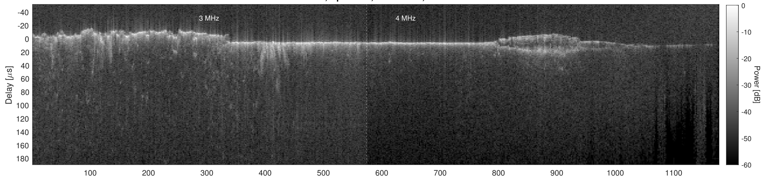
Orbit 5776, Cluttergram
